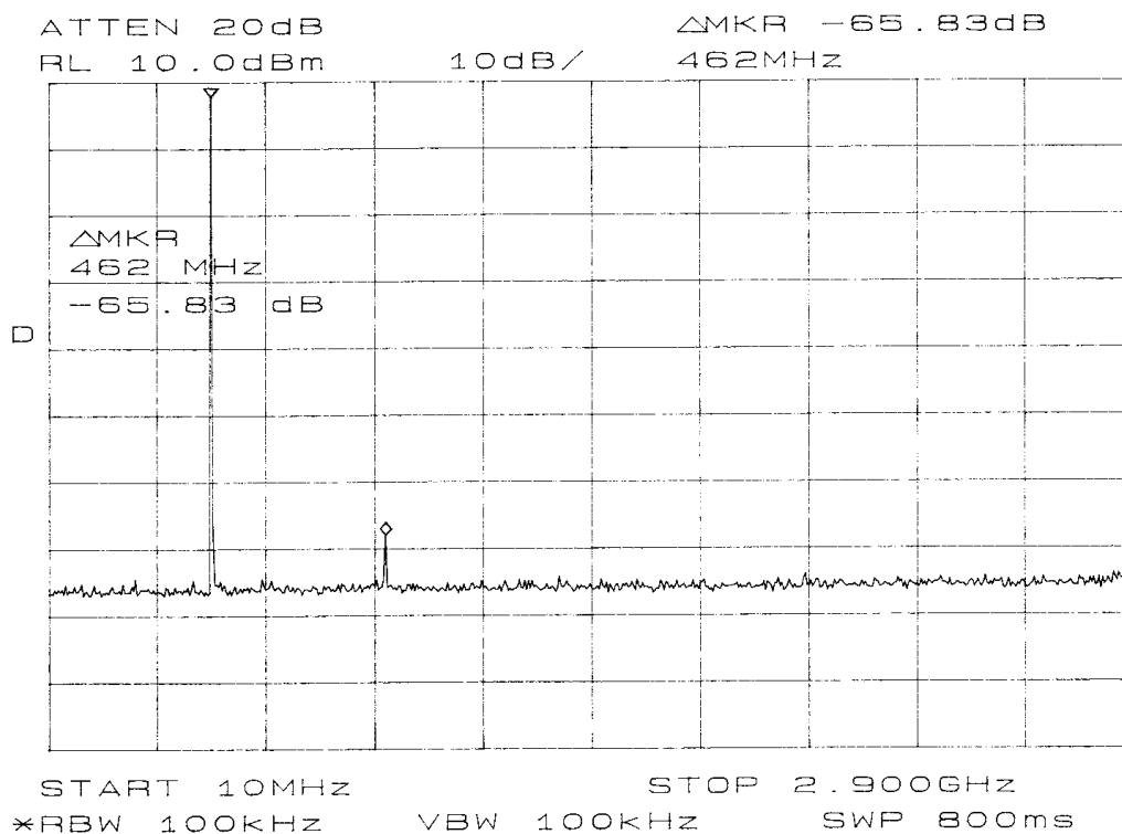
Figure 14: Emissions at Antenna Terminal (1W)
