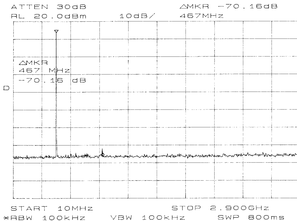
Figure 16: Emissions at Antenna Terminal (5W)
