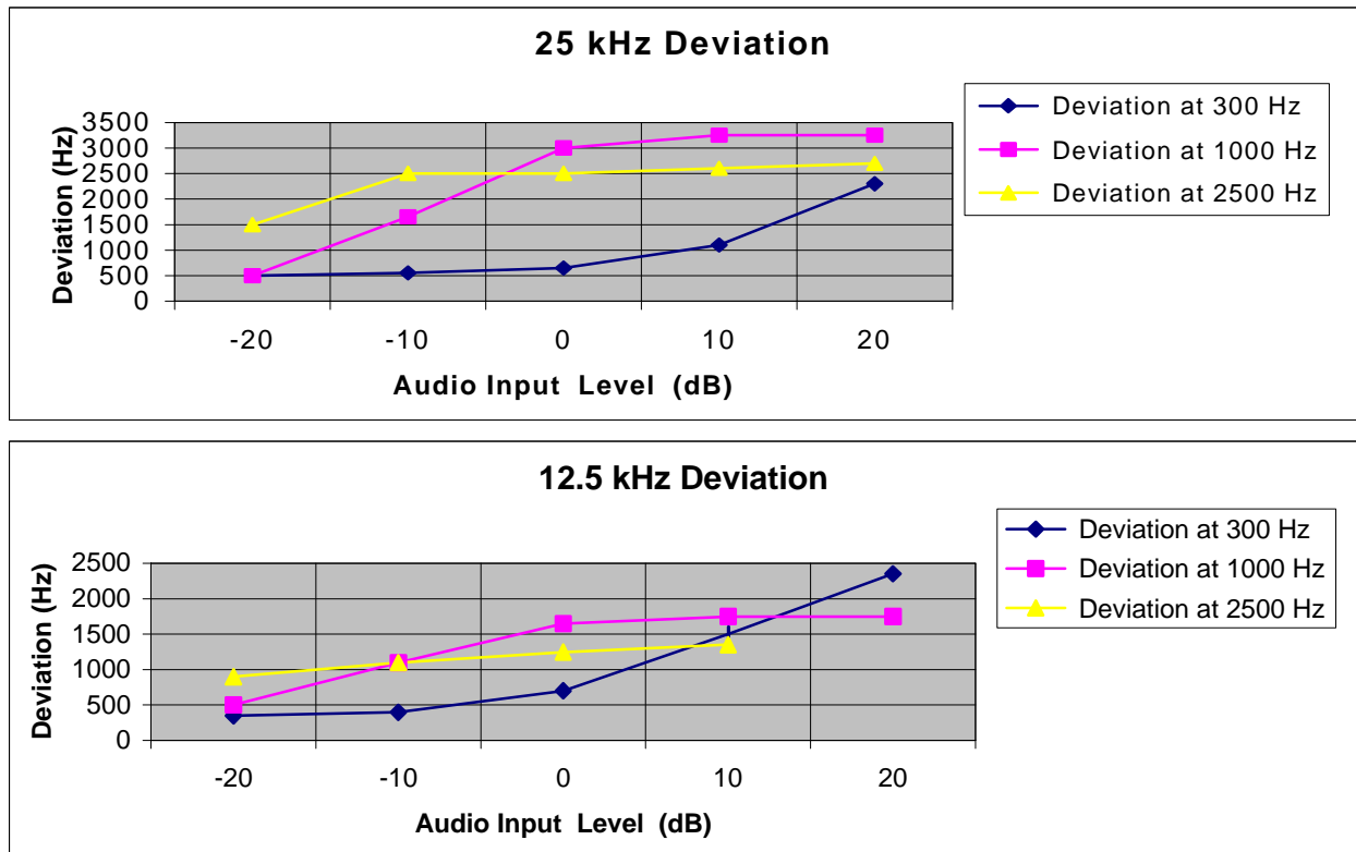
Figure 8: Deviation Characteristics.
