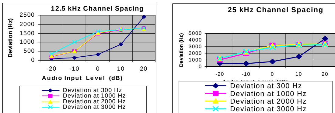
Figure 5: Deviation Characteristics.
