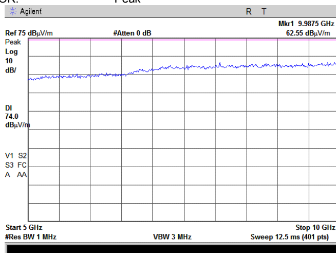
Plot 7.1.10 Radiated emission measurements from 5000 to 10000 MHz
