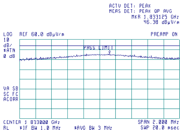
Plot 7.1.12 Radiated emission measurements at the second harmonic frequency
