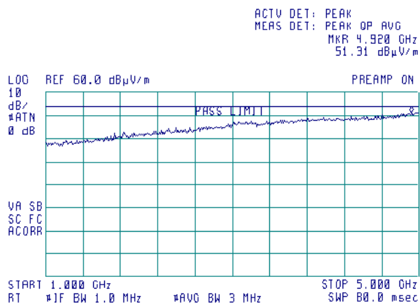
Plot 7.1.8 Radiated emission measurements from 1000 to 5000 MHz
