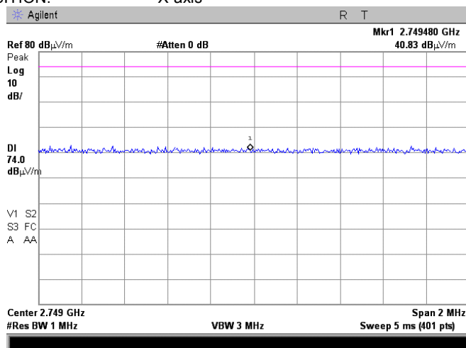
Plot 7.1.14 Radiated emission measurements at the fourth harmonic frequency
