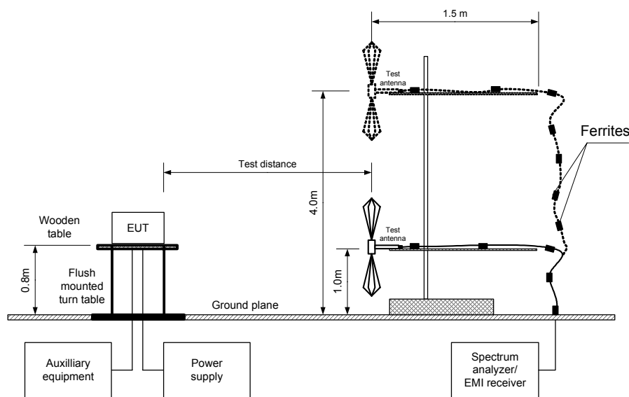
Figure 7.2.1 Band edge emission measurement set up
