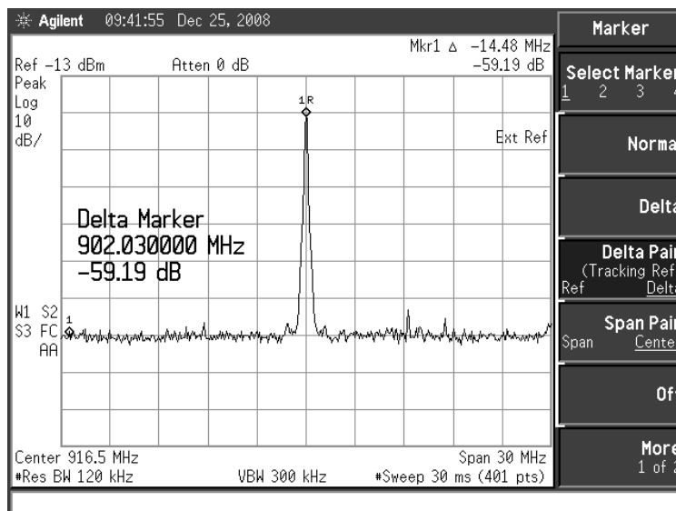
Plot 7.2.1 Low band edge emission test result
