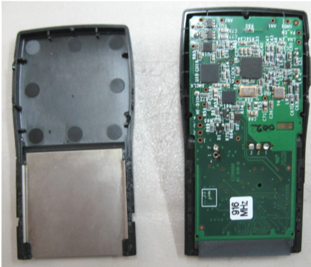
Photograph No.1 Master Handheld Terminal (MHHT) internal view
