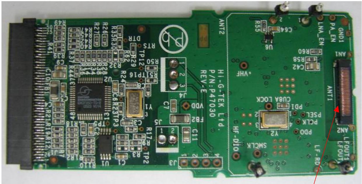
Photograph No.5 Master Handheld Terminal PCB second side view without HF antenna card
