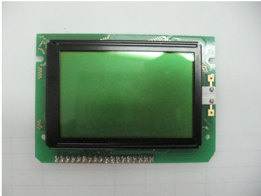
Figure 2 LCD Side 1
