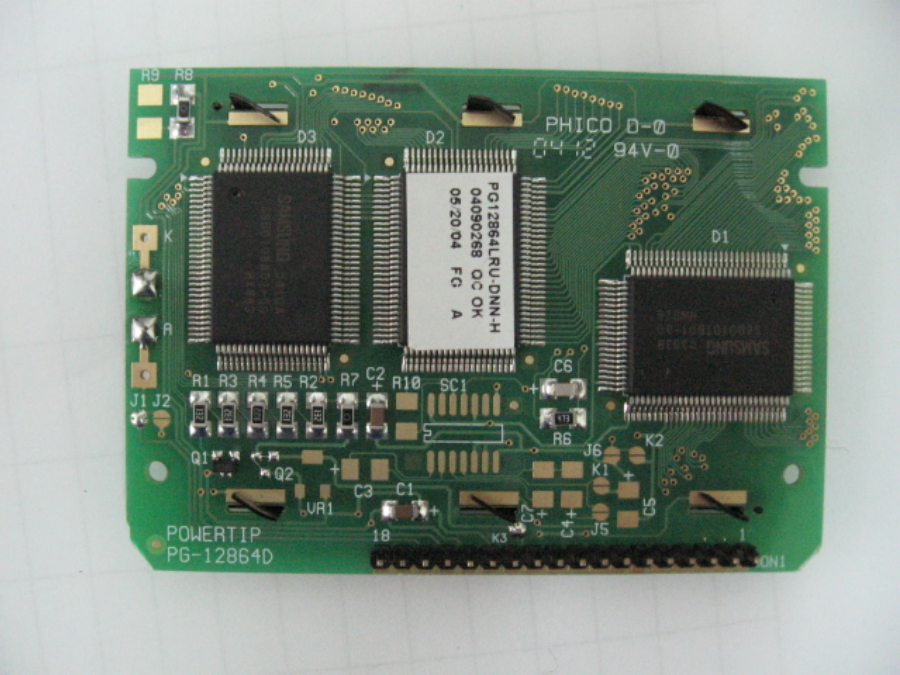
Figure 3 LCD Side 2
