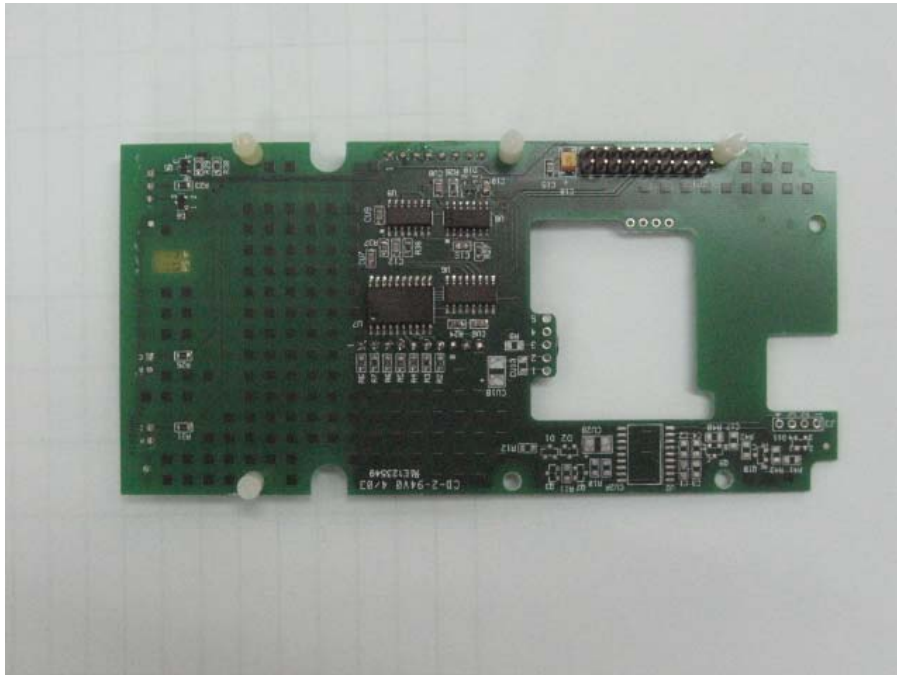
Figure 5 PCB 1 Print Side
