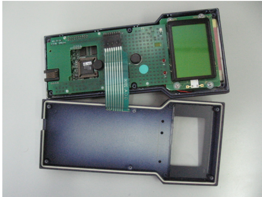
Figure Internal View
