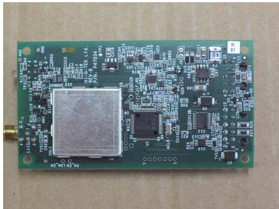
Figure 16 PCB Side 2
