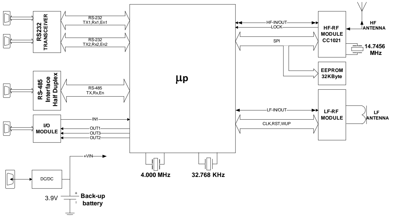
Figure 4. Block Diagram
