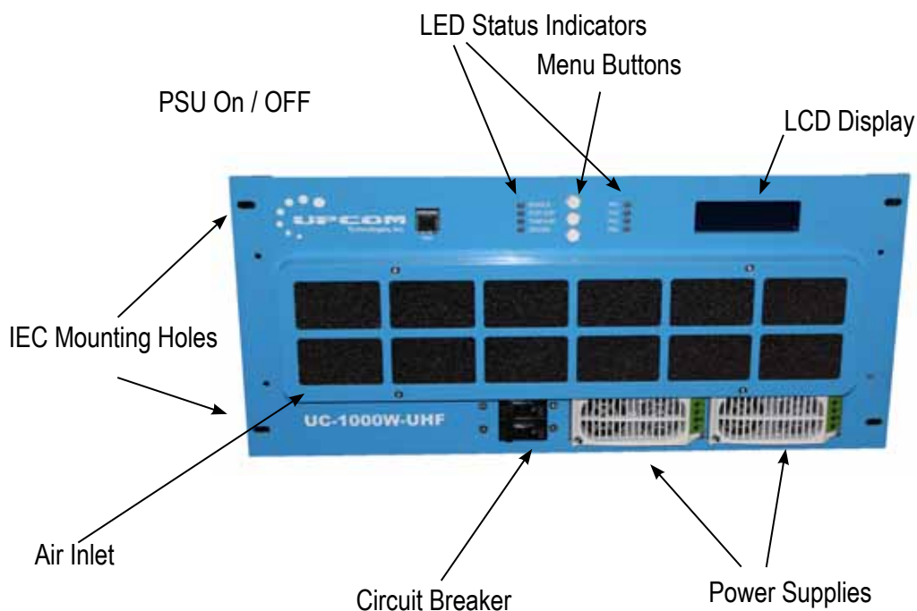
Figure 1.0 Amplifier Front
