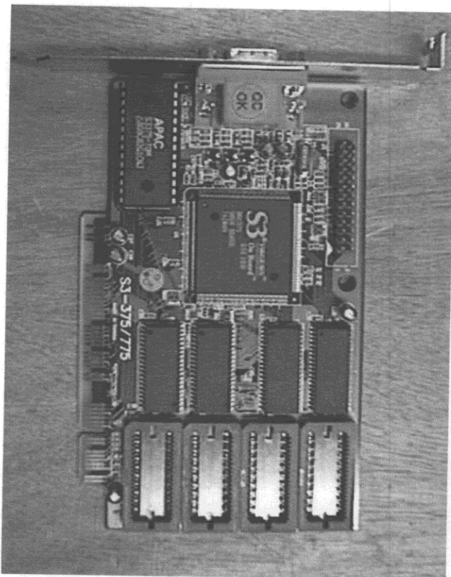
Photo 9 - Video Card - Component side
