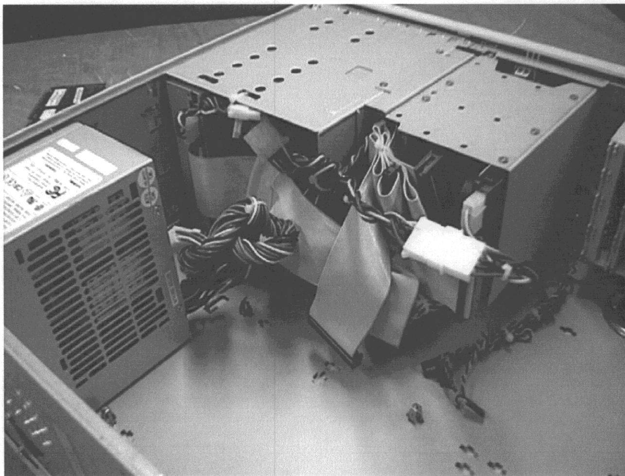
Photo 8 - Detail of Power Supply and power supply cables routing
