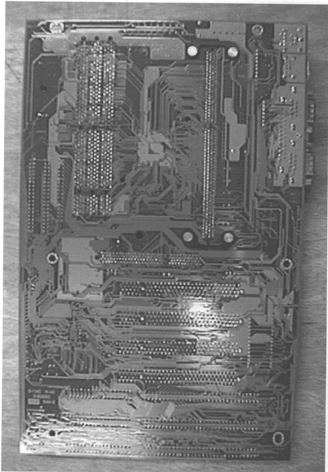
Photo 5 - Microtec Tower Personal Computer Mythus 6233 Main Board - Solder side view
