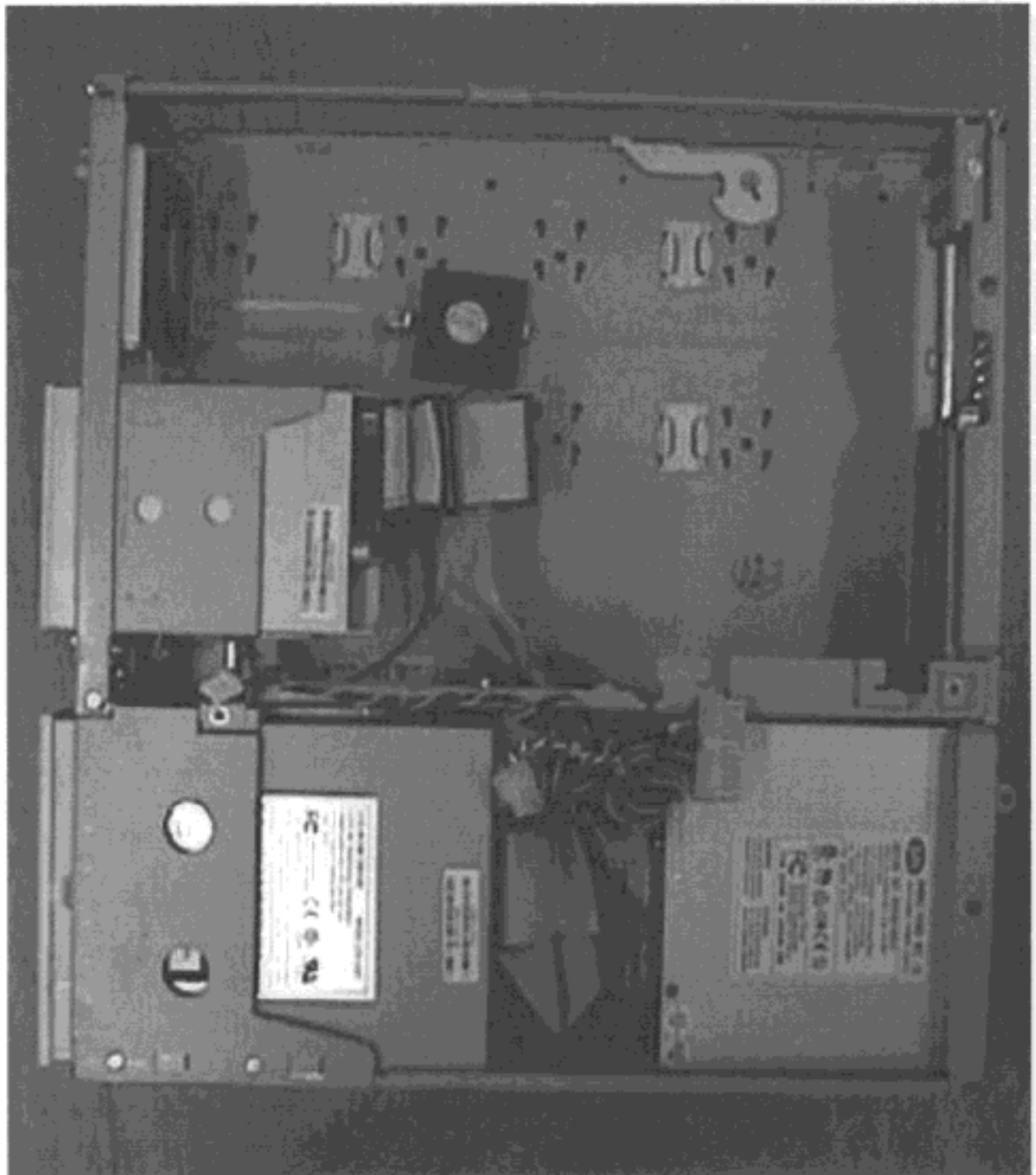
Photo 8 - Detailed view of the Microtec Desktop Personal Computer Mythus 6300 without the Main Board and Riser Card
