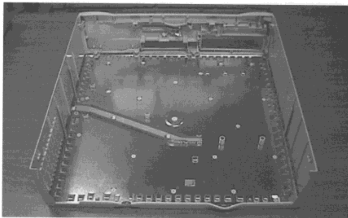
Photo 12 - Cabinet cover with pre mounted gasket
