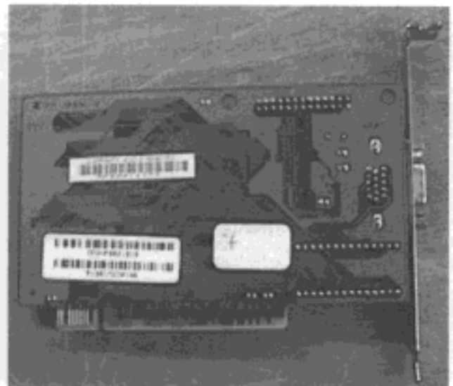
Photo 10 - Video Card - Solder side
