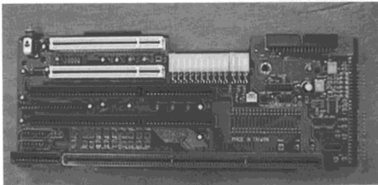
Photo 5 - Microtec Desktop Personal Computer Mythus 6300 Riser Card - Component side view
