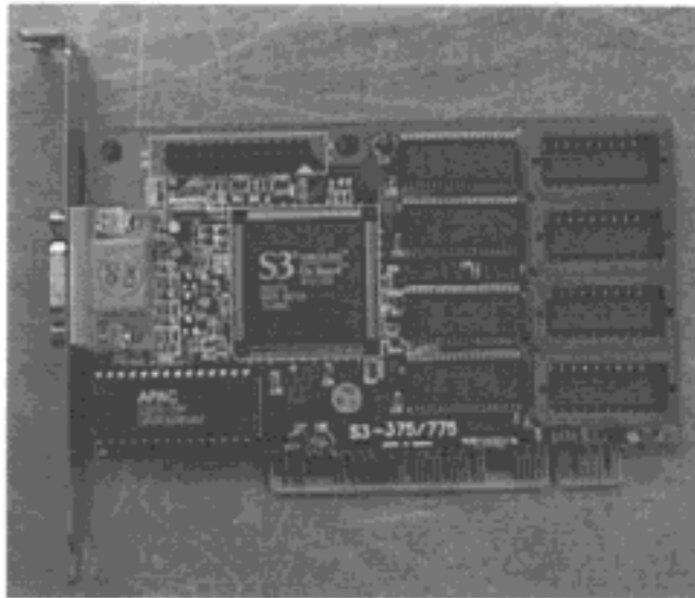
Photo 9 - Video Card - Component side
