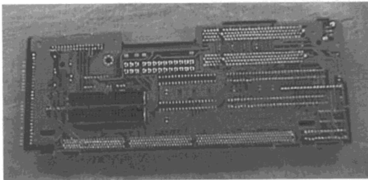
Photo 6 - Microtec Desktop Personal Computer Mythus 6300 Riser Card - Solder side view
