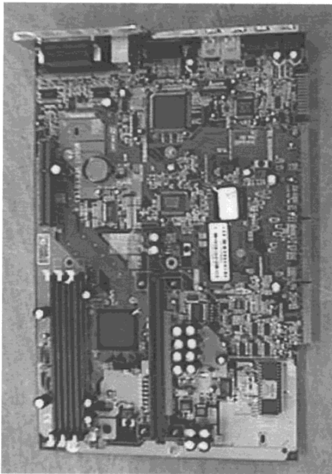
Photo 3 - Microtec Desktop Personal Computer Mythus 6300 Main Board - Component side view
