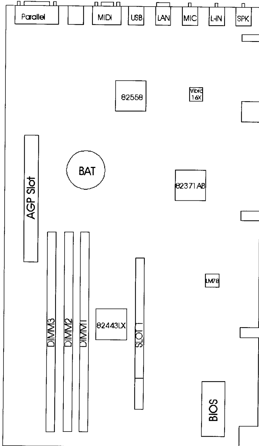
Figure 1 - Microtec Desktop Personal Computer Mythus 6300 Main Board drawing
