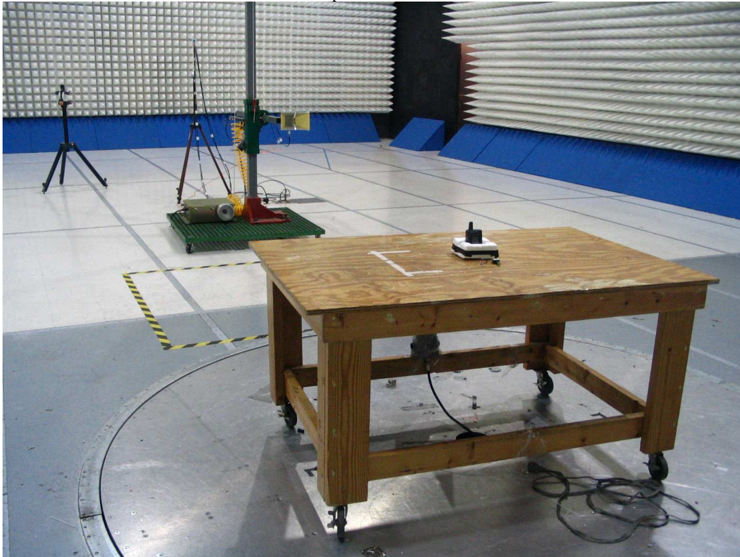
Transmitter Spurious Emissions – Back
