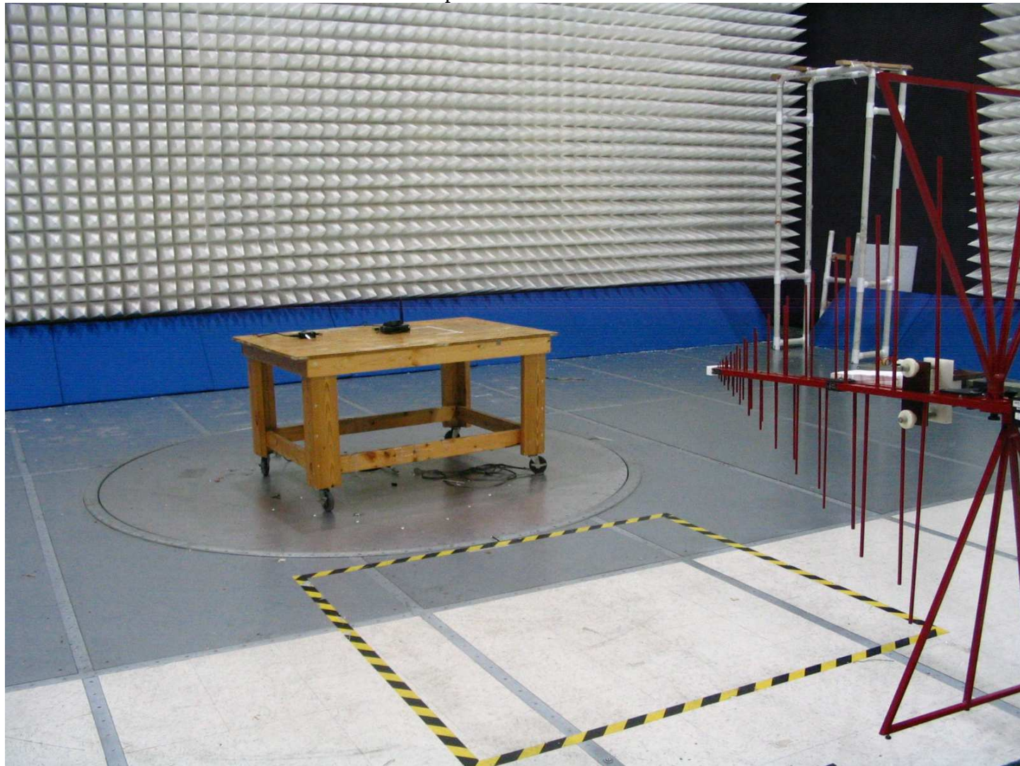
Receiver Spurious Emissions – Front
