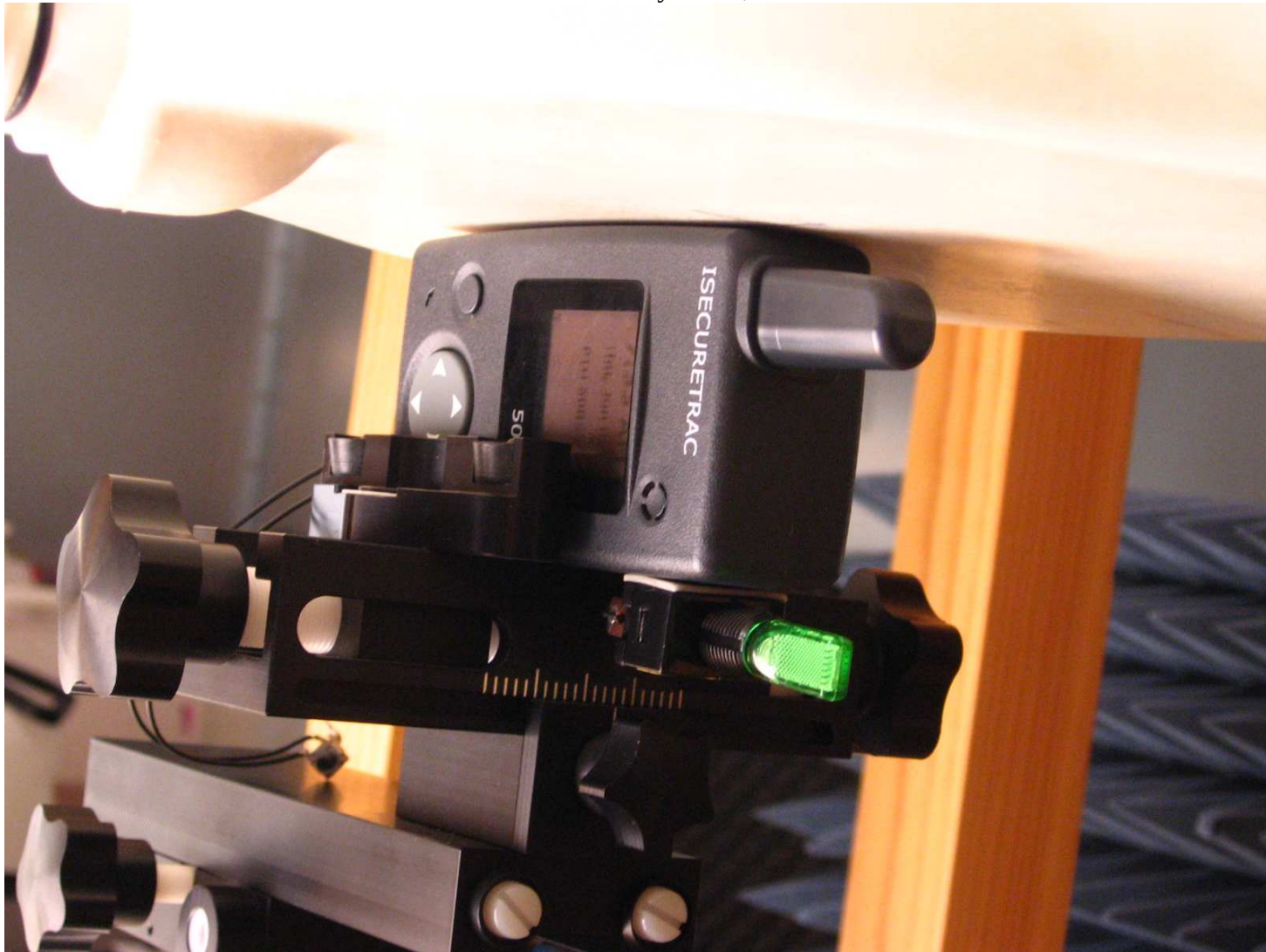
SAR Test – Body Mode, Left
