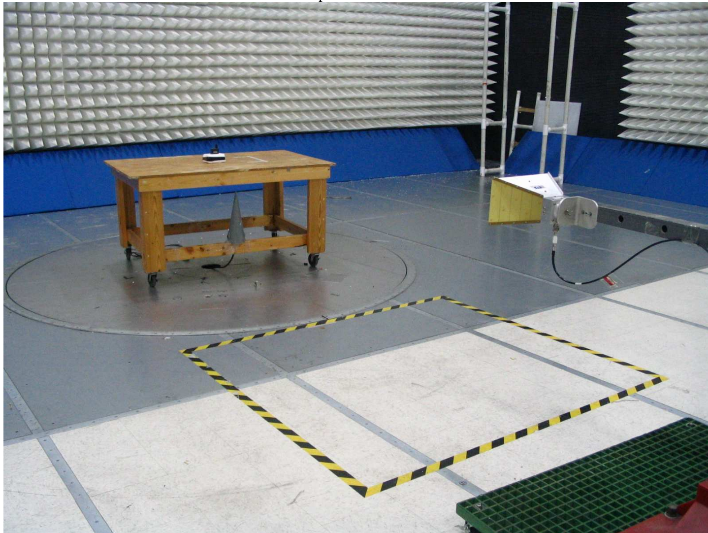
Transmitter Spurious Emissions – Front
