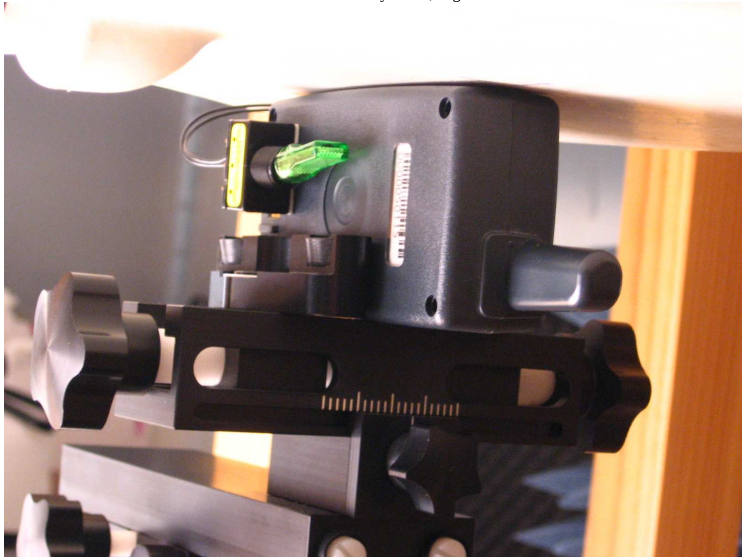
SAR Test – Body Mode, Right
