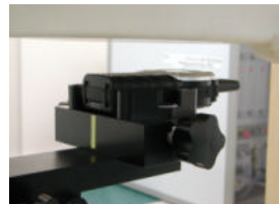
Figure 11. Mouth Face SAR Test Setup
