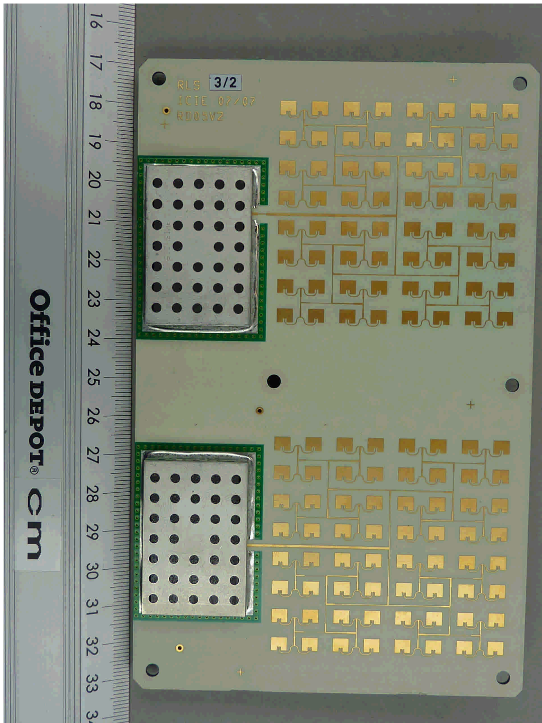
110464_i.jpg RLS, PCB, bottom view
