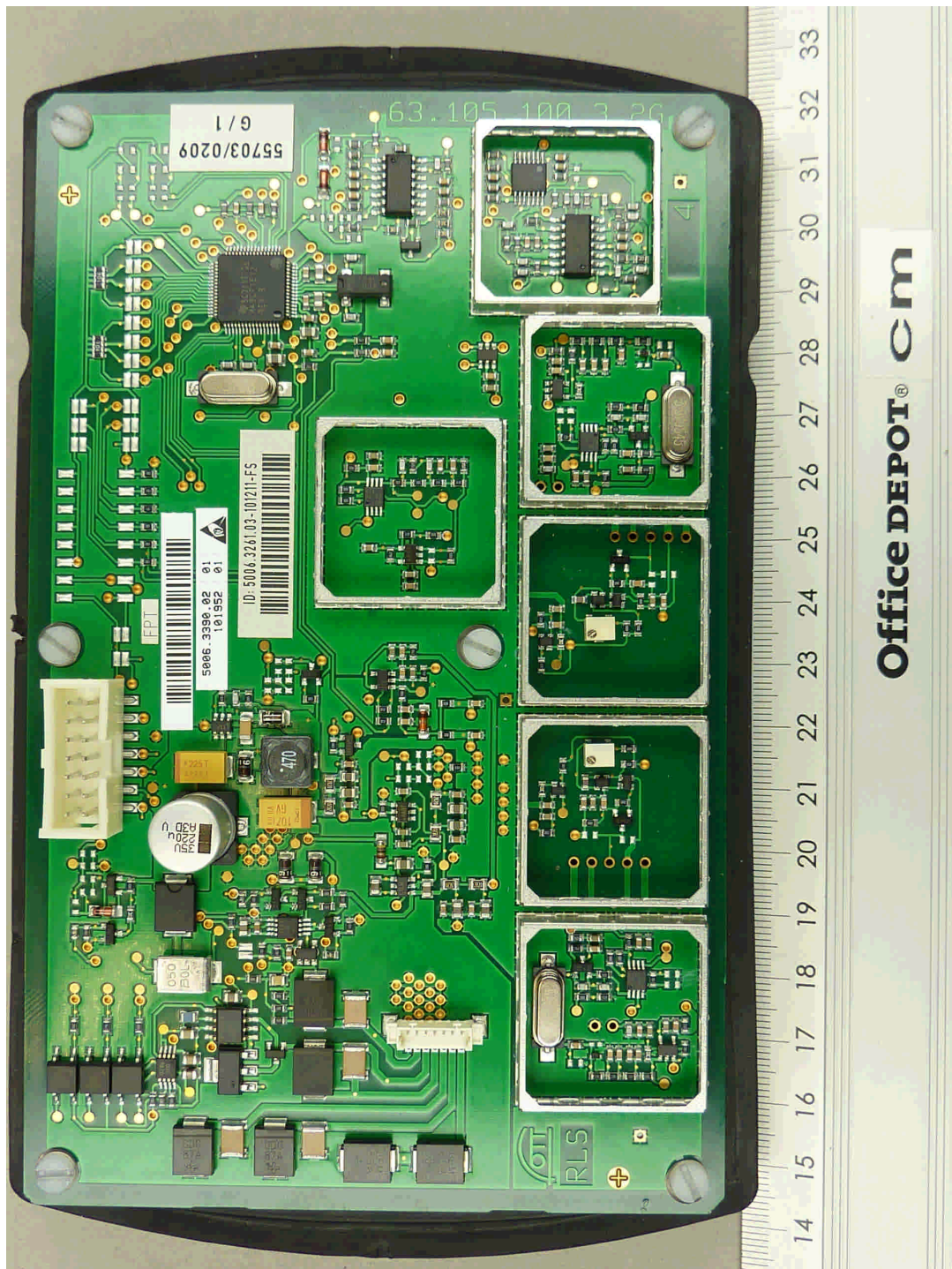
110464_g.jpg RLS, PCB, top view, covers removed
