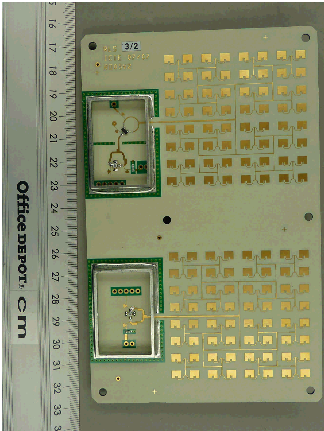
110464_h.jpg RLS, PCB, bottom view, covers removed
