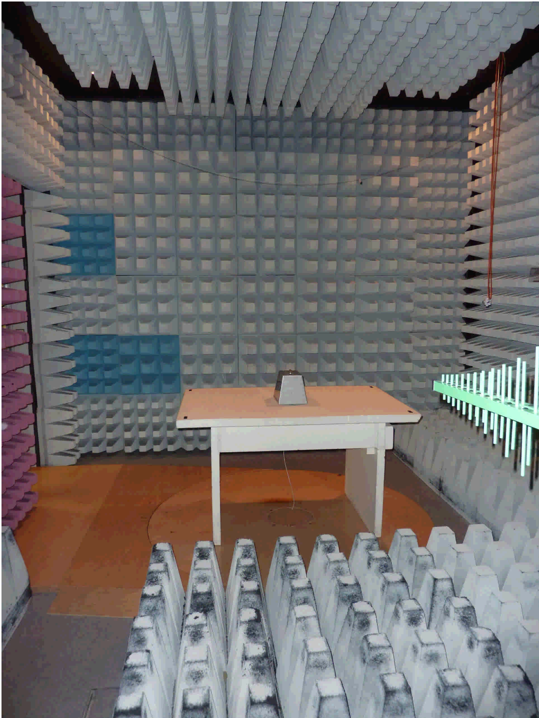
110464_4.jpg RLS, test set-up fully anechoic chamber
