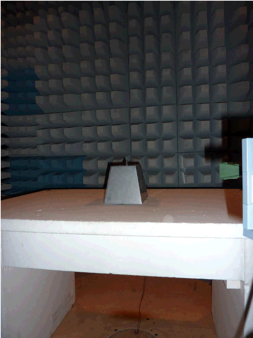
110464_10.jpg RLS, test set-up fully anechoic chamber
