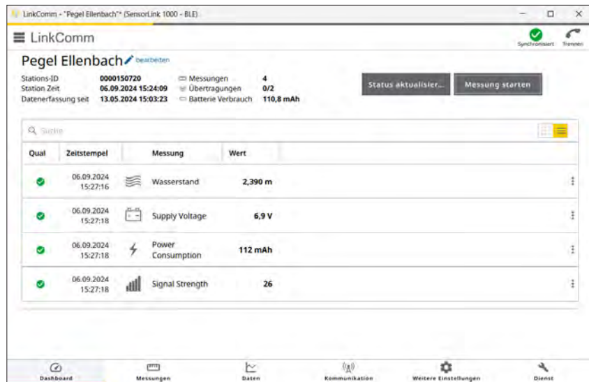
Fig. 15: Setting of OTT SensorLink 1000 operating parameters – Dashbord of operating software "LinkComm".
