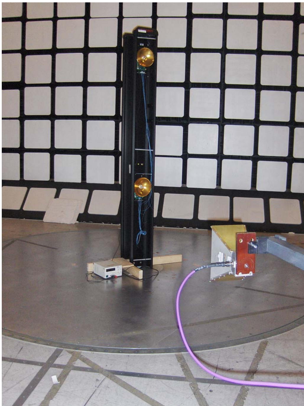
Radiated Emissions @ 3 m (Tx/Rx)
