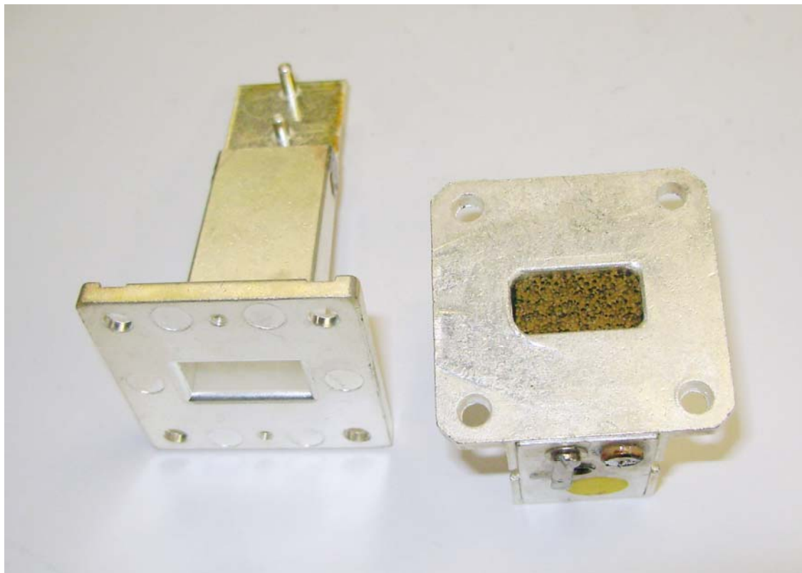
Transmit unit
