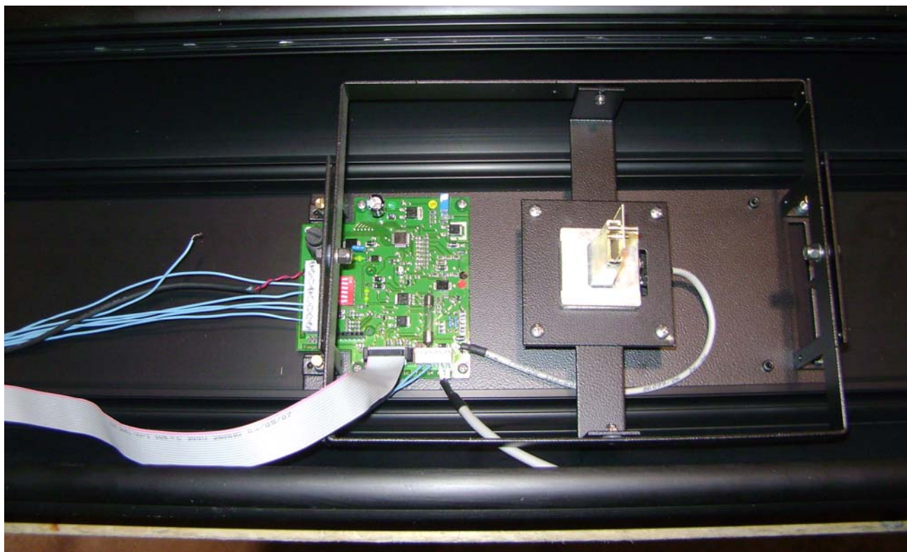
Transmit unit
