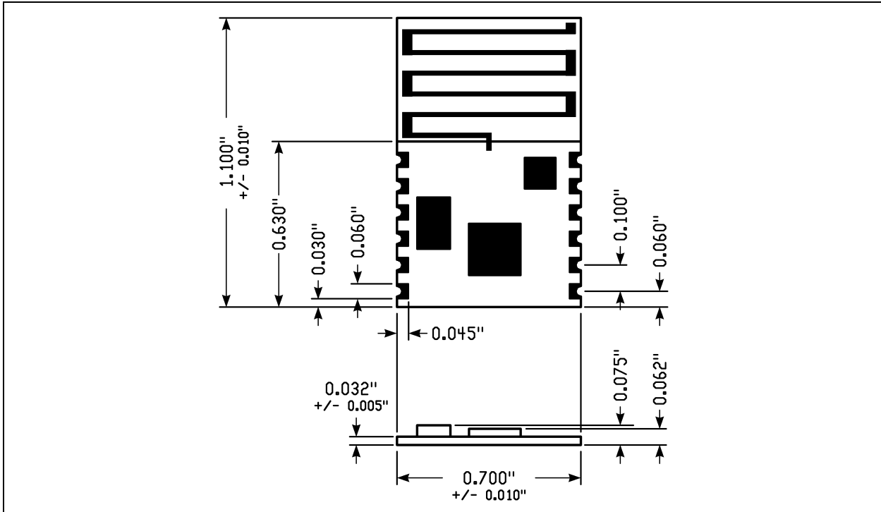
FIGURE 1-3: MODULE DETAILS
