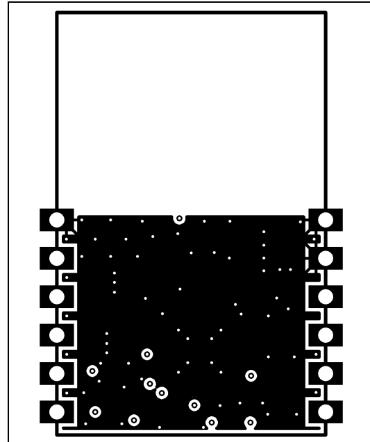
FIGURE 2-5: LAYER 2 — GROUND PLANE
