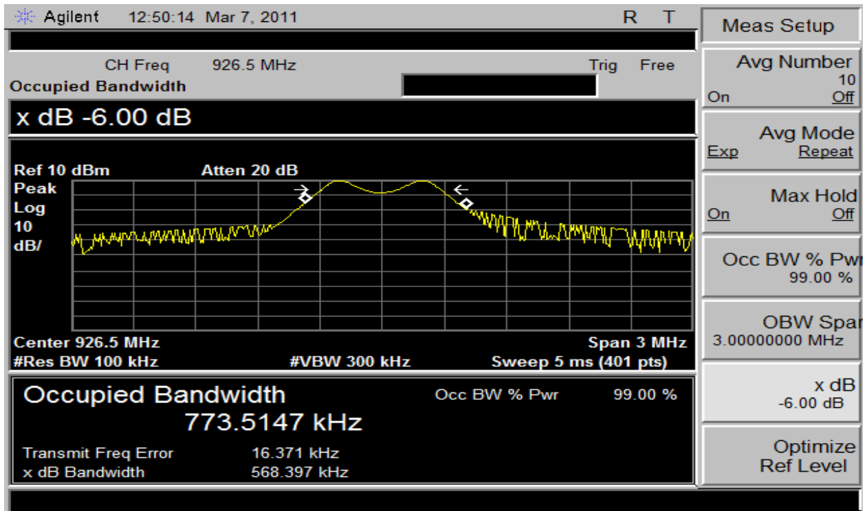
Plot 7 – Highest Channel – 6dB BW FSK Modulation 50kbps Data Rate
