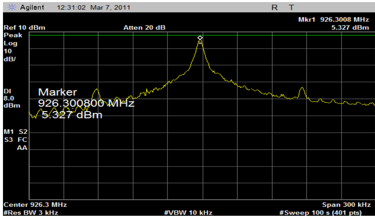
Plot 29 – Highest Channel (PSD) 2kbps Data Rate
