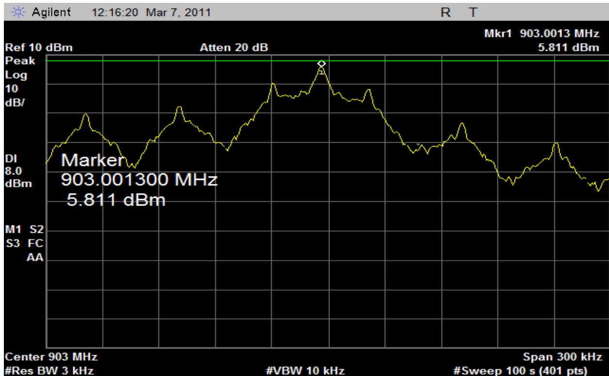
Plot 24 – Lowest Channel (PSD) 50kbps Data Rate
