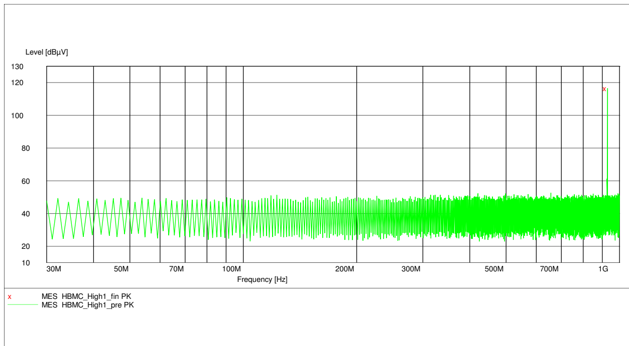
Plot 18 – Highest Channel (30MHz to 1GHz)
