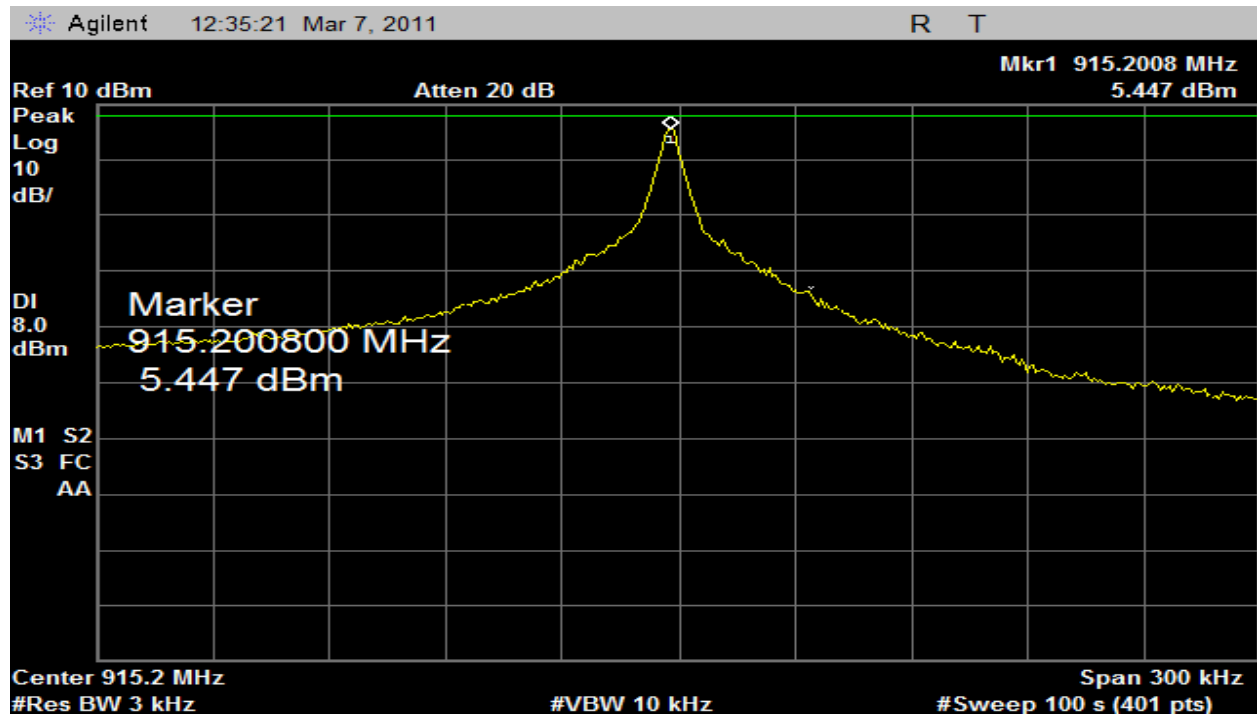
Plot 28 – Middle Channel (PSD) 2kbps Data Rate
