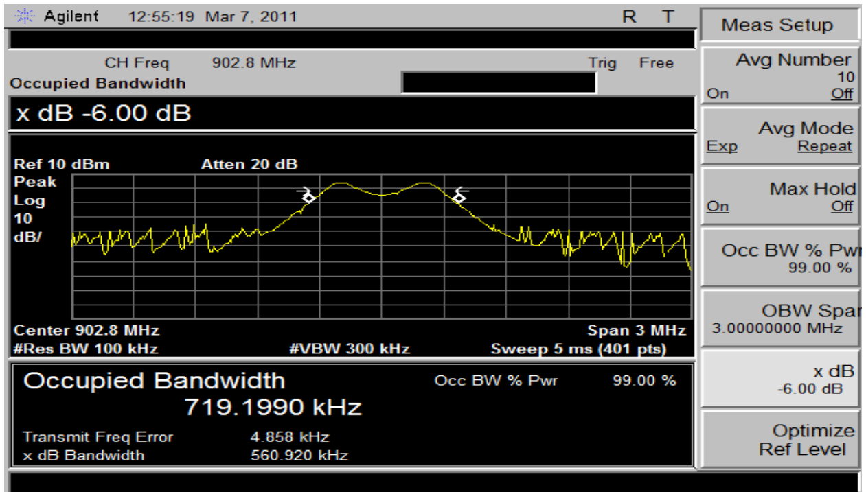
Plot 8 – Lowest Channel – 6dB BW FSK Modulation 2kbps Data Rate
