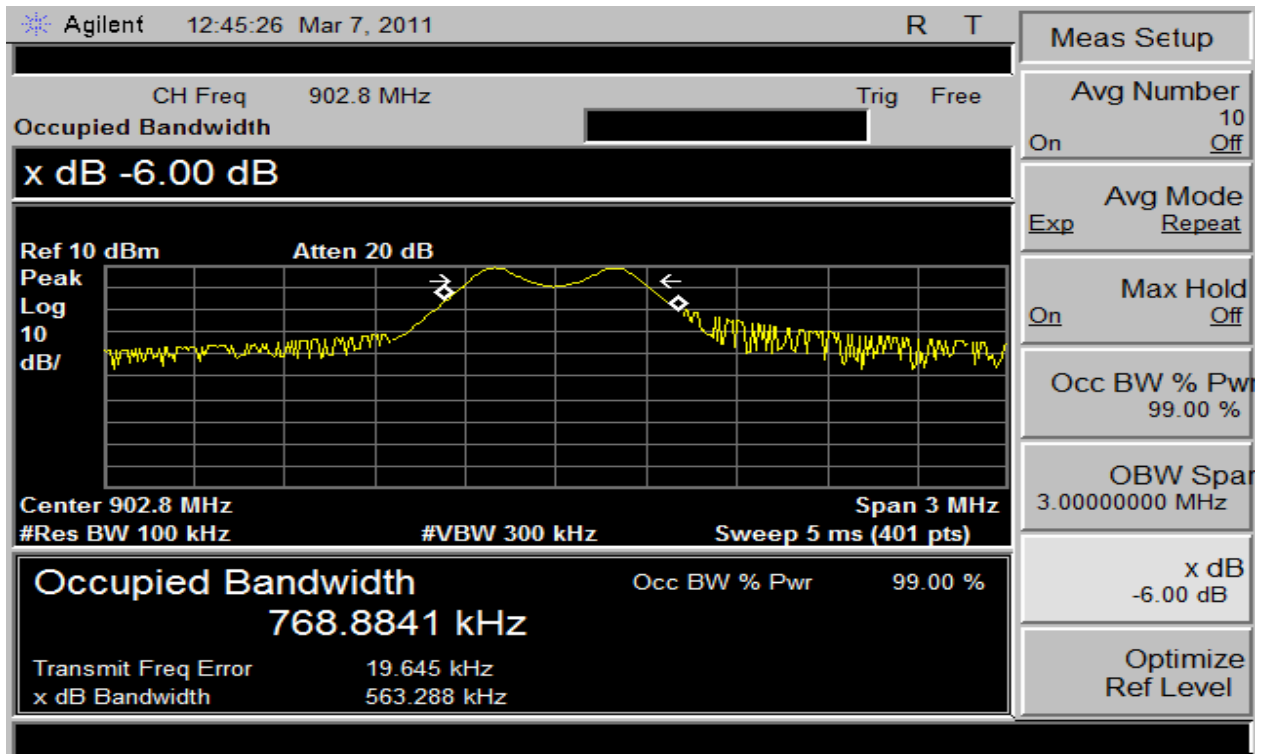
Plot 5 – Lowest Channel – 6dB BW FSK Modulation 50kbps Data Rate
