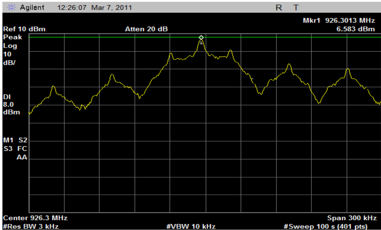
Plot 26 – Highest Channel (PSD) 50kbps Data Rate
