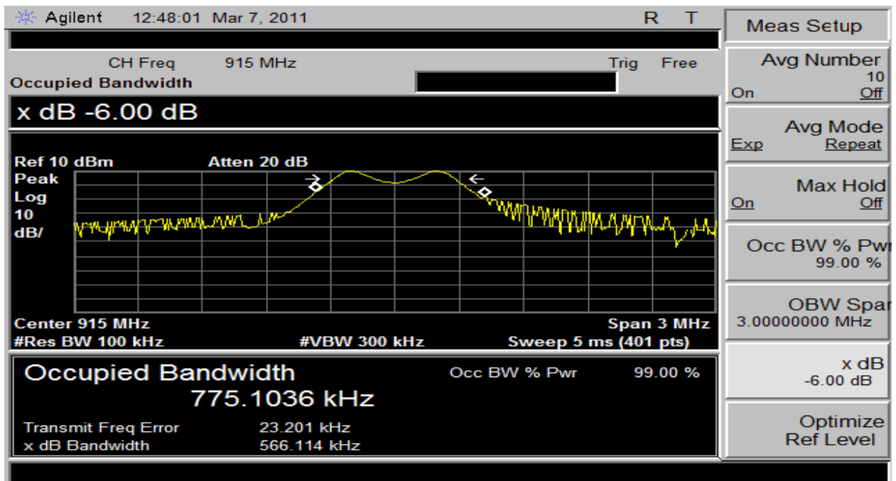
Plot 6 – Middle Channel – 6dB BW FSK Modulation 50kbps Data Rate
