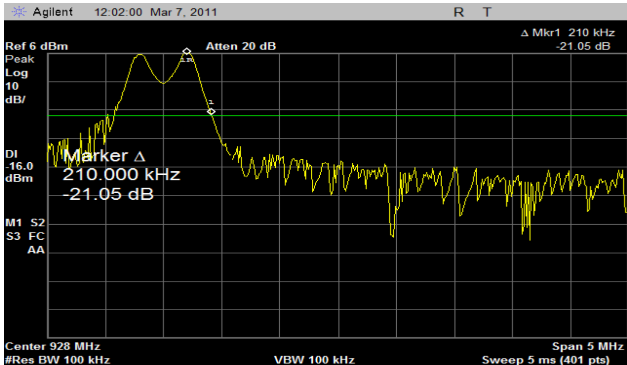
Plot 23 – Highest Channel (Band Edge) 2kbps Data Rate
