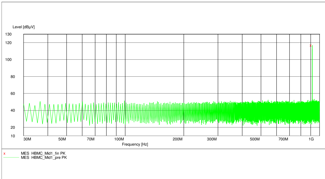
Plot 16 – Middle Channel (30MHz to 1GHz)
