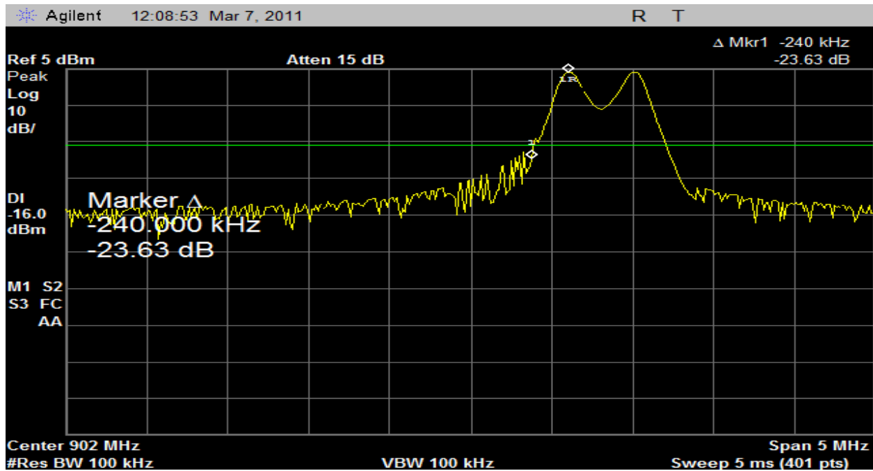
Plot 22 – Lowest Channel (Band Edge) 2kbps Data Rate
