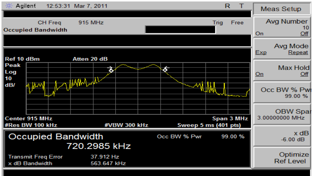
Plot 9 – Middle Channel – 6dB BW FSK Modulation 2kbps Data Rate
