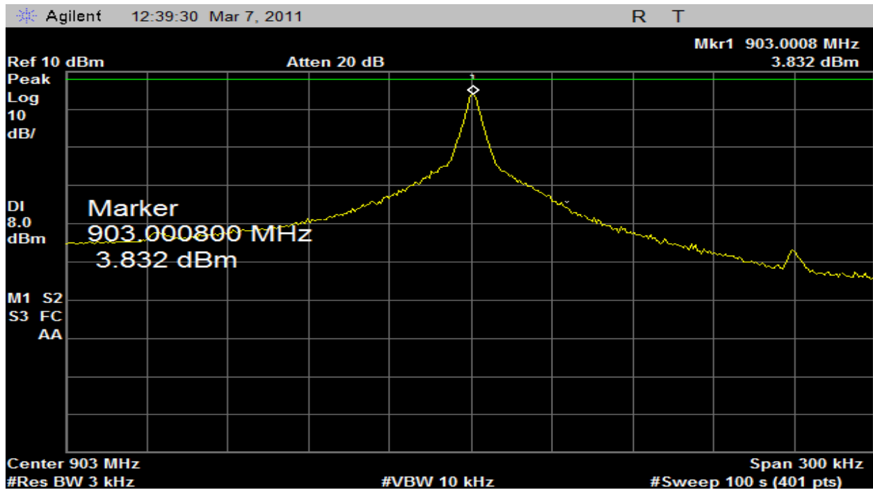
Plot 27 – Lowest Channel (PSD) 2kbps Data Rate
