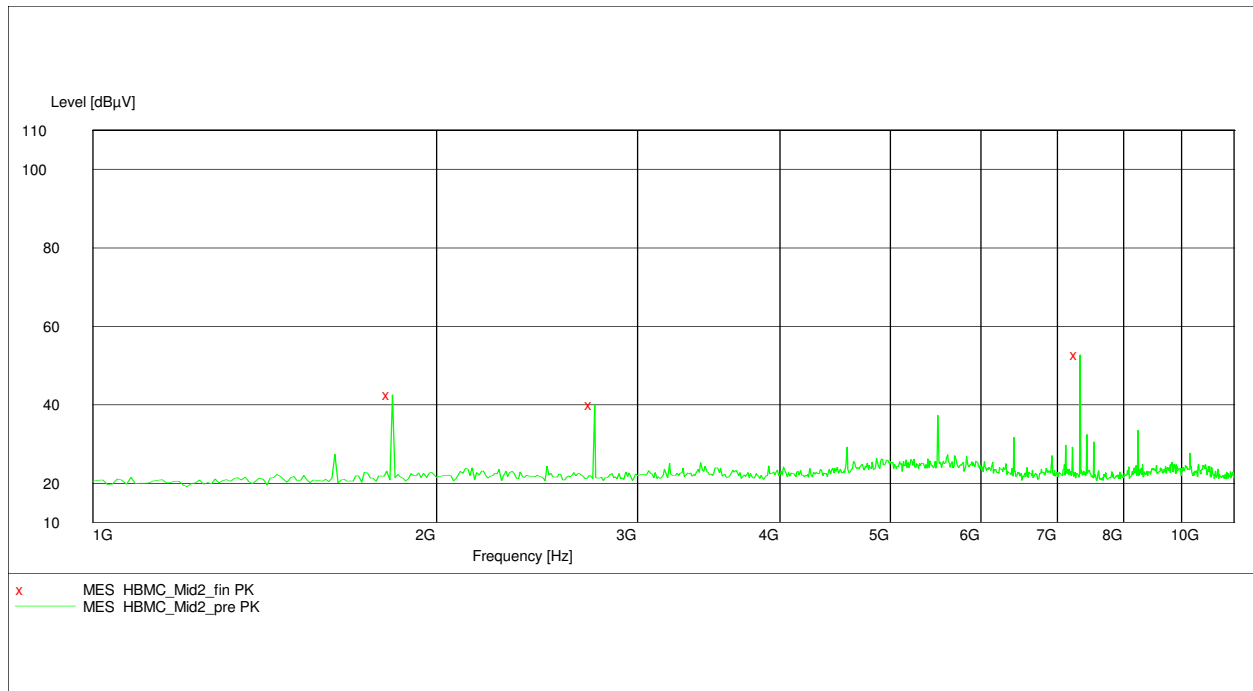
Plot 17 – Middle Channel (1GHz to 10GHz)
