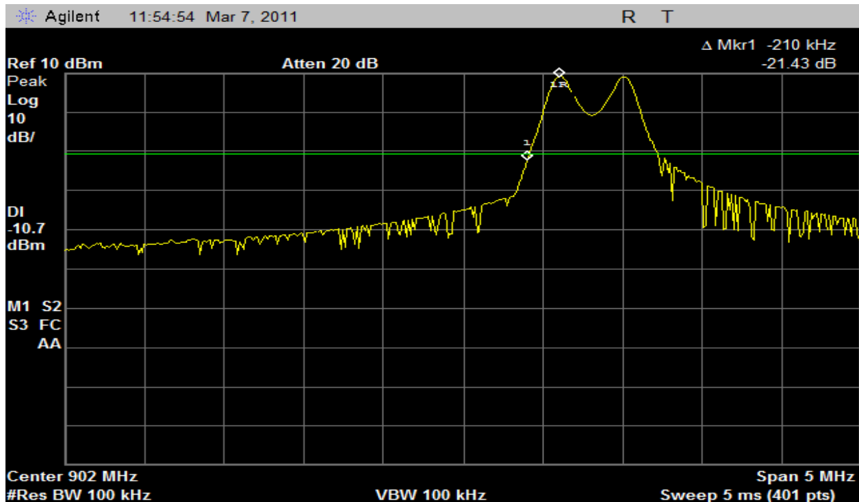
Plot 20 – Lowest Channel (Band Edge) 50kbps Data Rate
