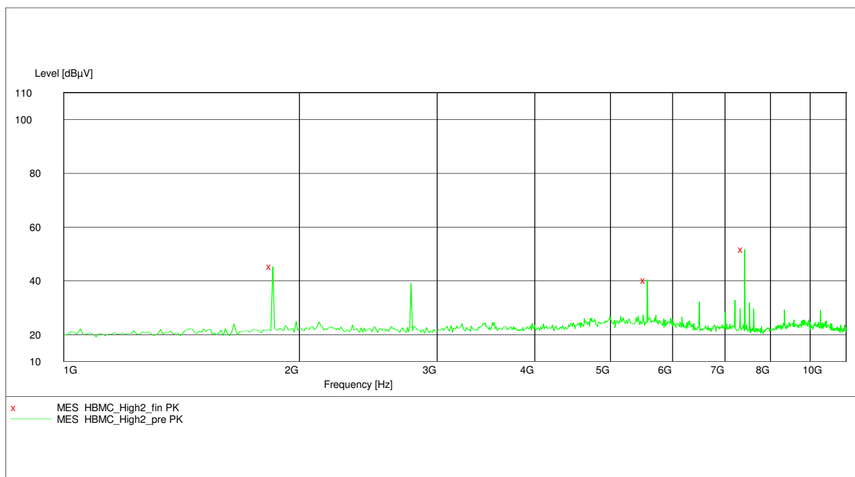
Plot 19 – Highest Channel (1GHz to 10GHz)
