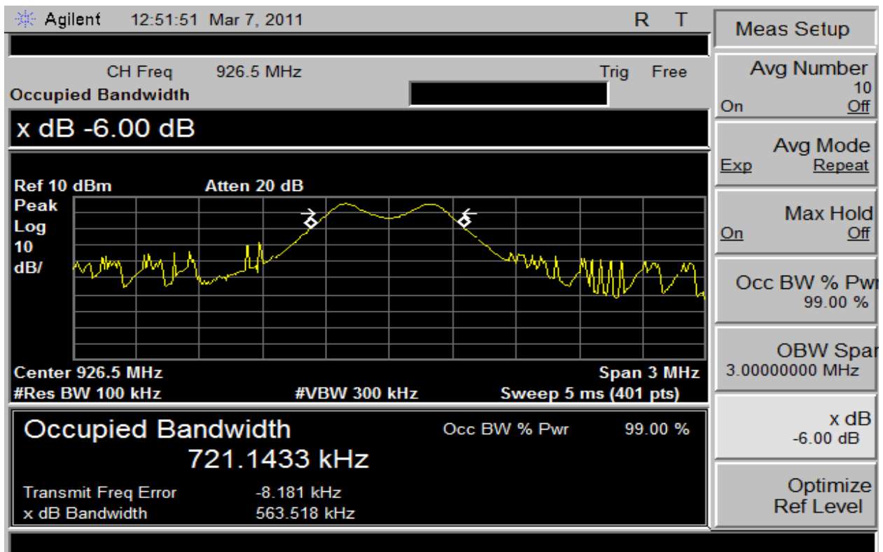
Plot 10 – Highest Channel – 6dB BW FSK Modulation 2kbps Data Rate
