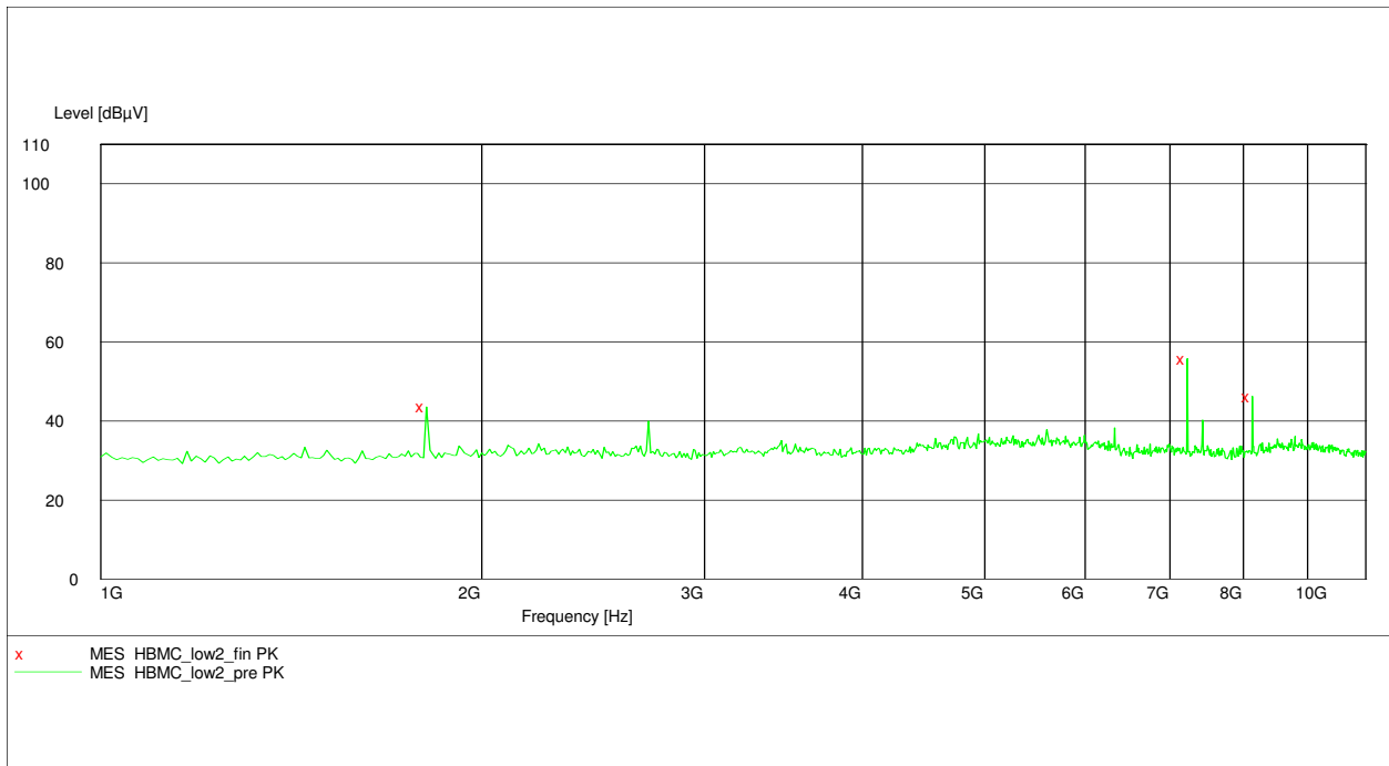
Plot 15 – Lowest Channel (1GHz to 10GHz)
