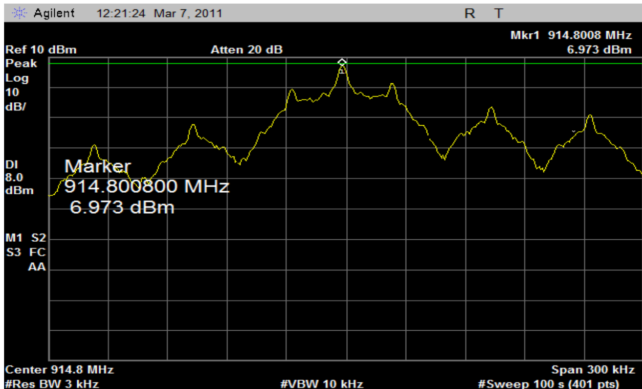
Plot 25 – Middle Channel (PSD) 50kbps Data Rate
