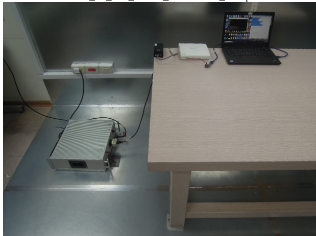
FCC_15_247_WLAN_Conduction_Setup
