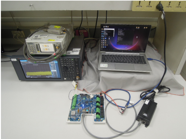
FCC_15_247_WLAN_Conducted_setup
