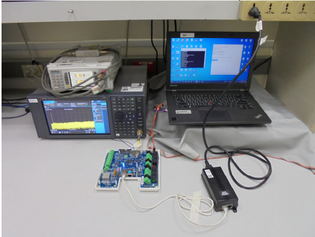
FCC_15_247_BT_Conducted_setup
