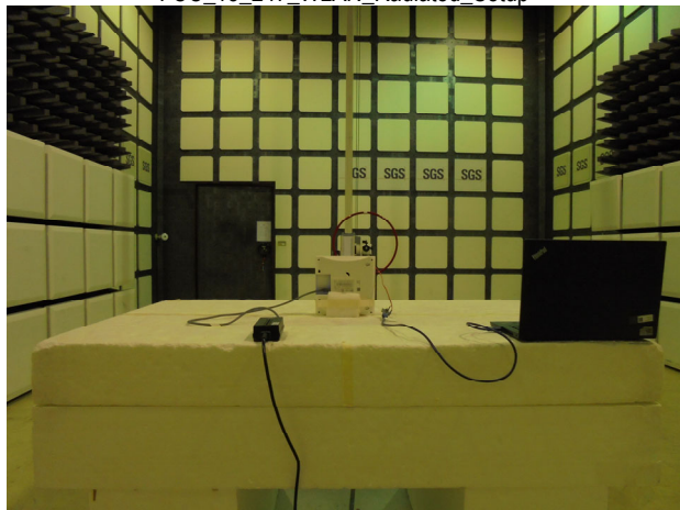
FCC_15_247_WLAN_Radiated_Setup
