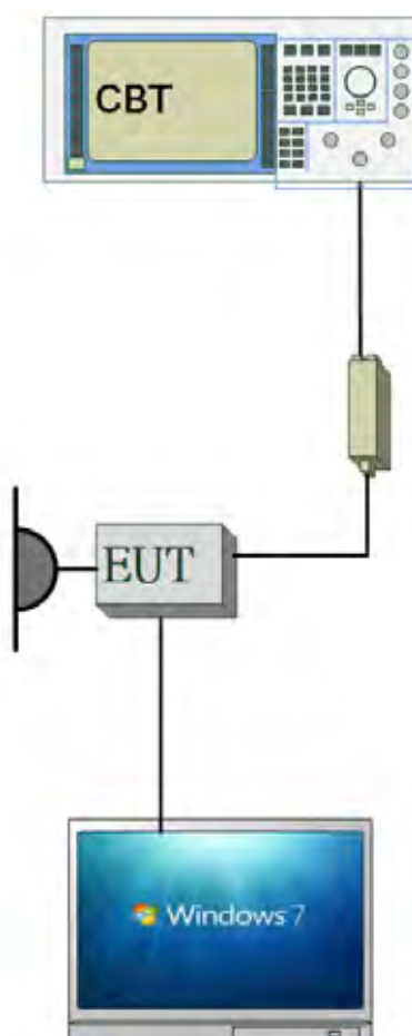
Fig. 2-2 Conducted (Antenna Port) Configuration
