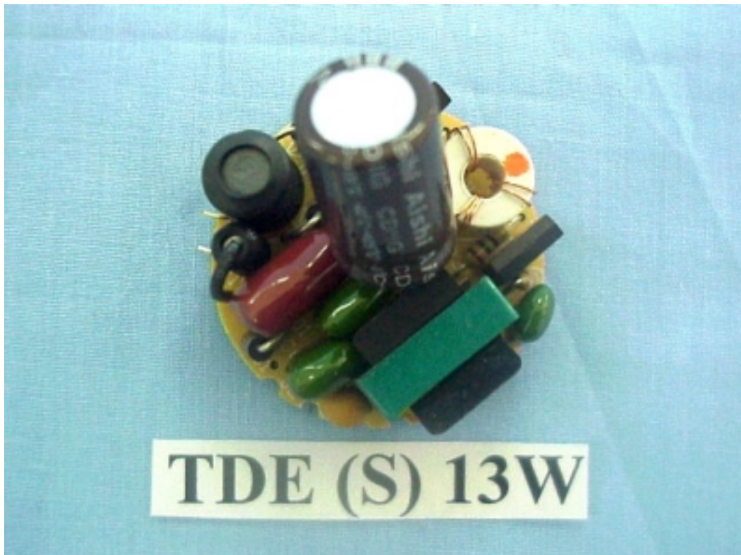
FIGURE 4 ENERGY SAVING LAMP (M/N: TDE (S) 13W) MAIN BOARD (COMPONENT SIDE)
