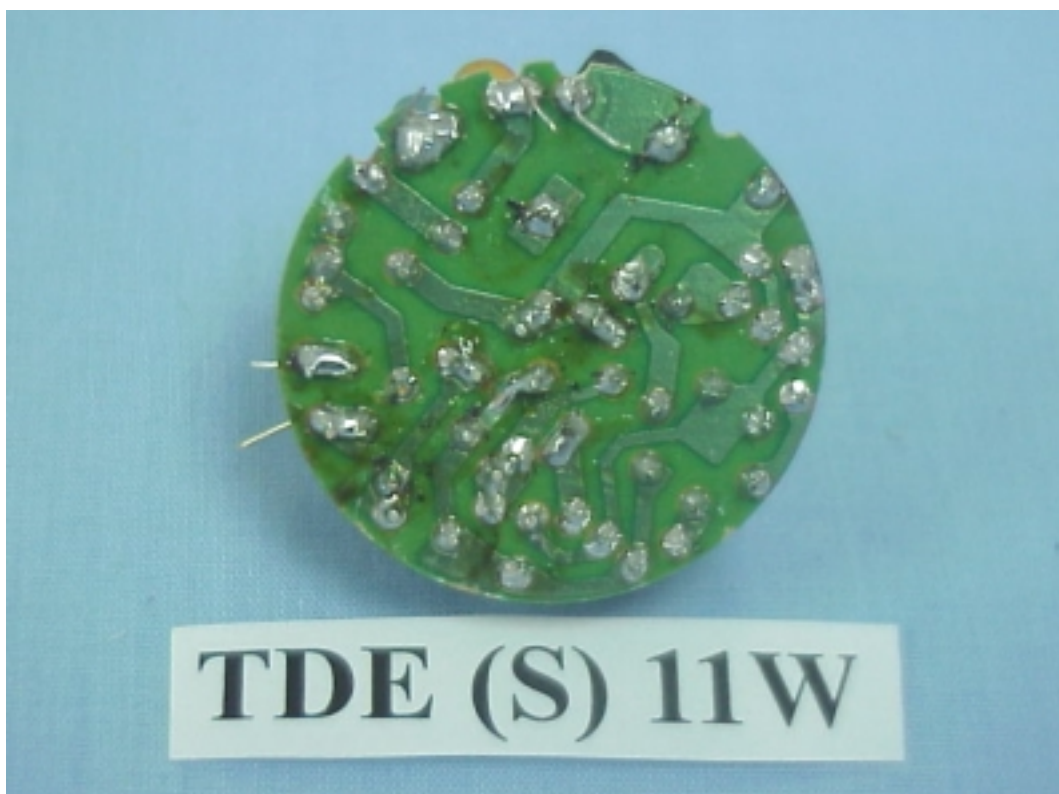
FIGURE 3 ENERGY SAVING LAMP (M/N: TDE (S) 11W) MAIN BOARD (SOLDERED SIDE)
