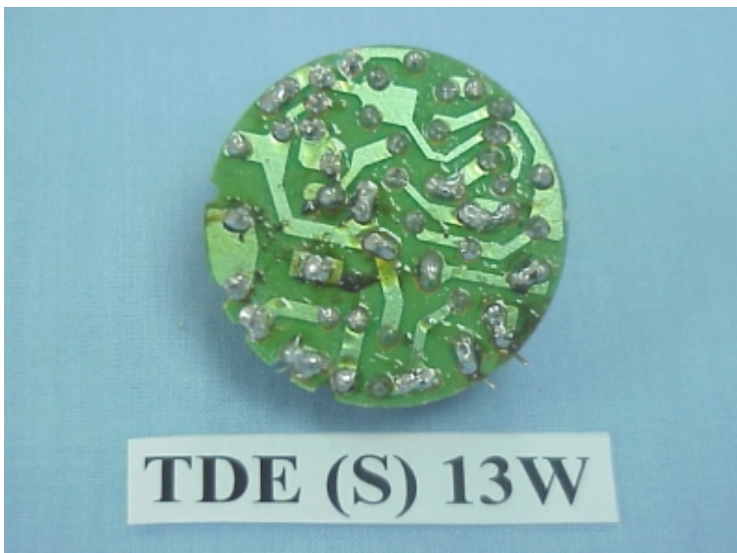
FIGURE 5 ENERGY SAVING LAMP (M/N: TDE (S) 13W) MAIN BOARD (SOLDERED SIDE)
