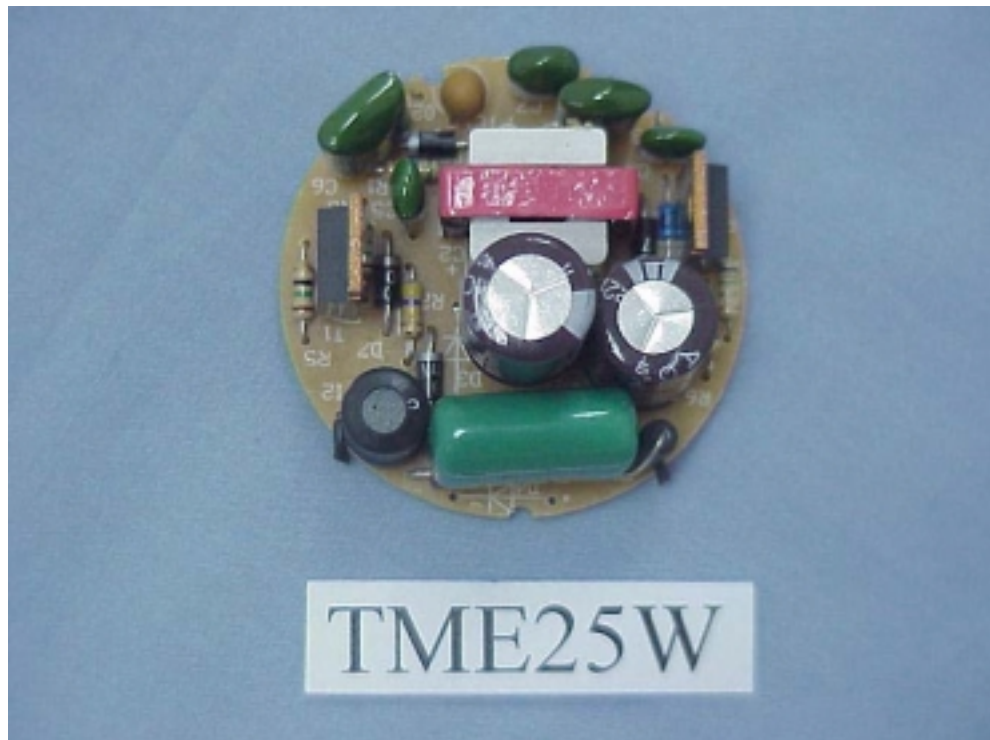
Figure 6 ENERGY SAVING LAMP (M/N: TME25W) MAIN BOARD (COMPONENT SIDE)
