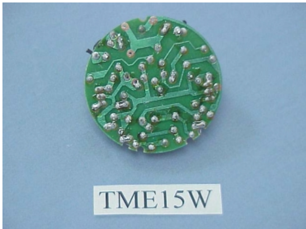
Figure 3 ENERGY SAVING LAMP (M/N: TME15W) MAIN BOARD (SOLDERED SIDE)
