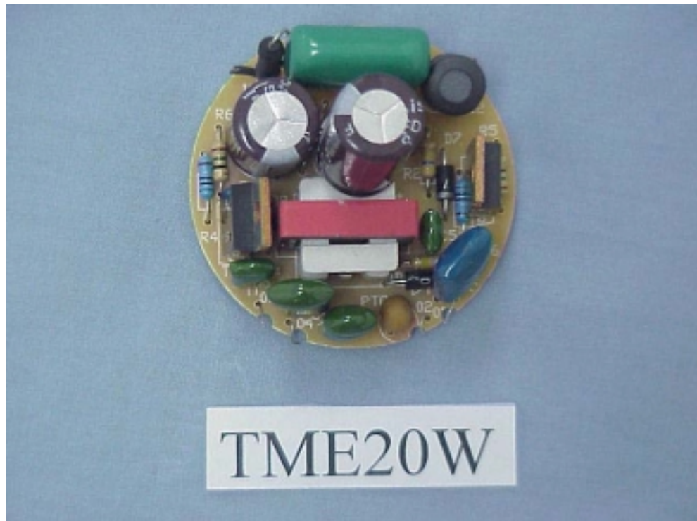
Figure 4 ENERGY SAVING LAMP (M/N: TME20W) MAIN BOARD (COMPONENT SIDE)
