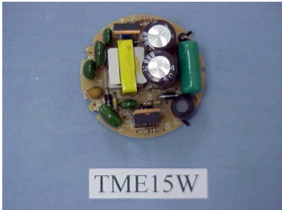
Figure 2 ENERGY SAVING LAMP (M/N: TME15W) MAIN BOARD (COMPONENT SIDE)
