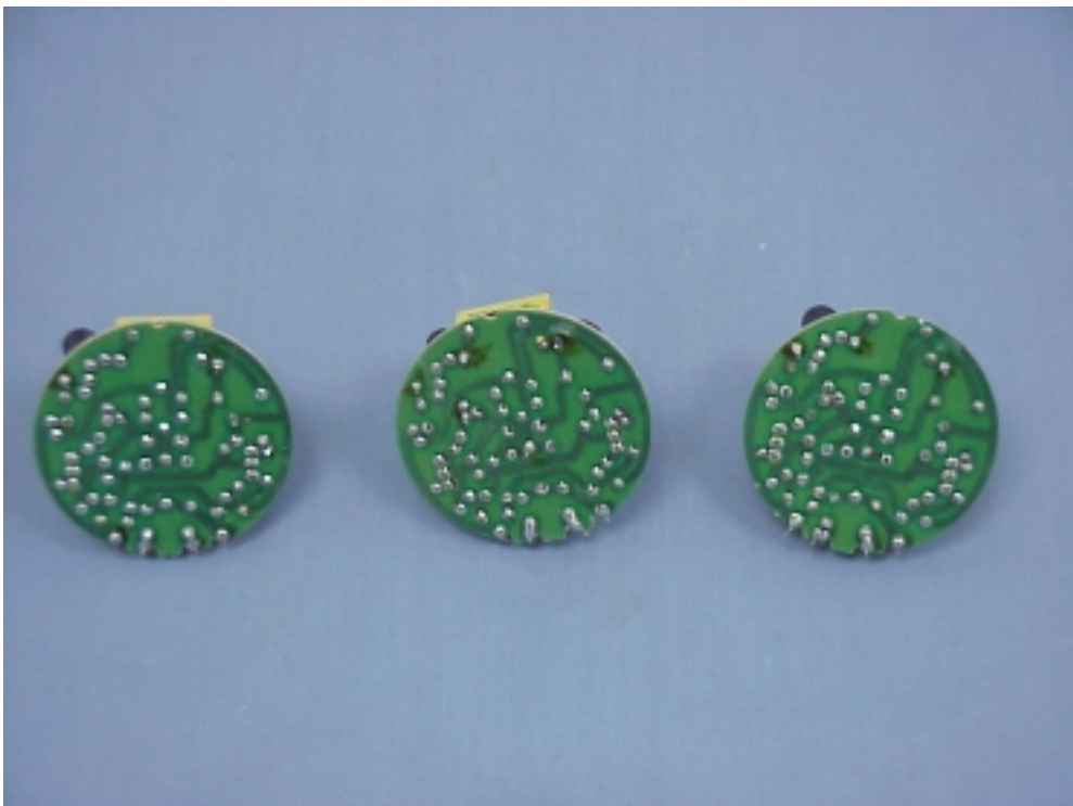
Figure 4 Energy Saving Lamp (M/N: TME15W, TME20W, TME25W) Main Board (Soldered Side)
