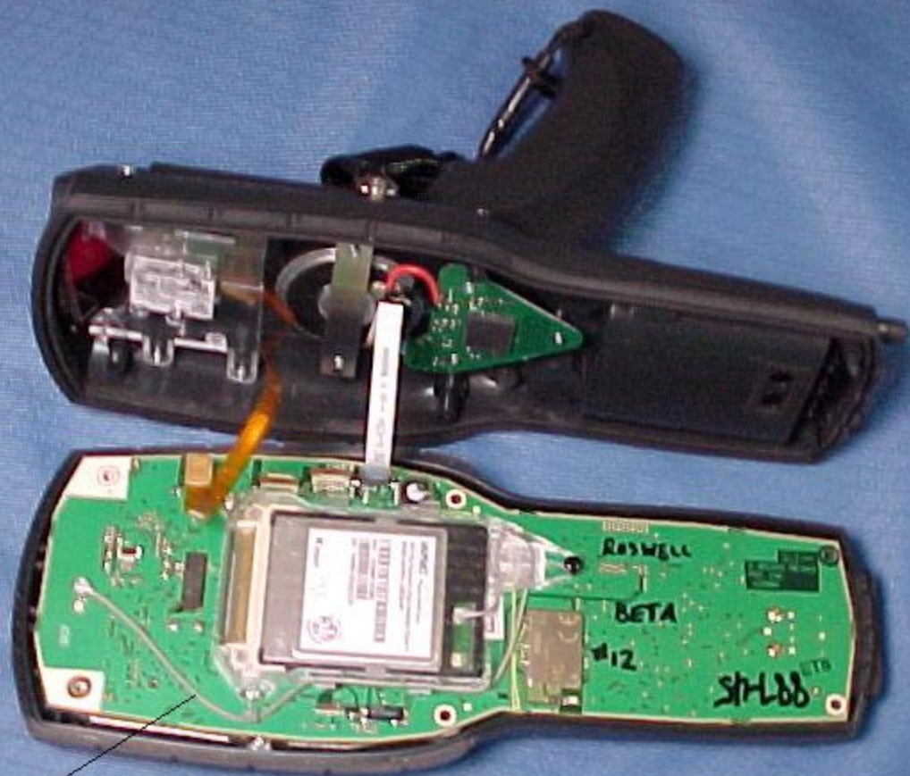
802.11 antenna cable
