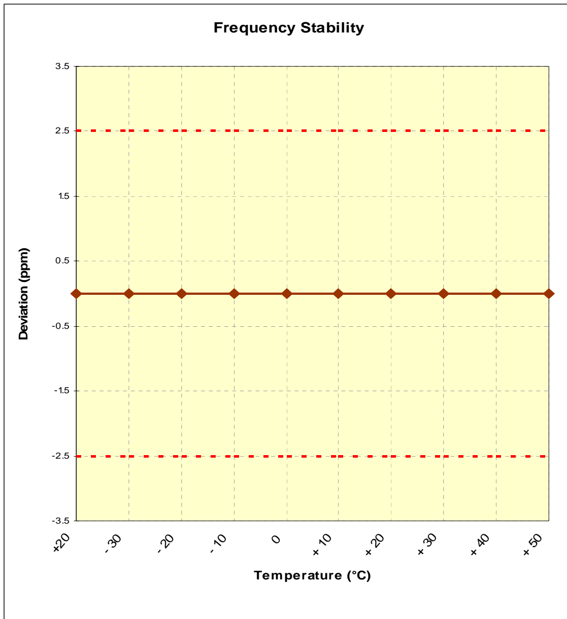
Figure 6-2. Frequency Stability Graph (Cellular CDMA Mode – Ch. 384)
