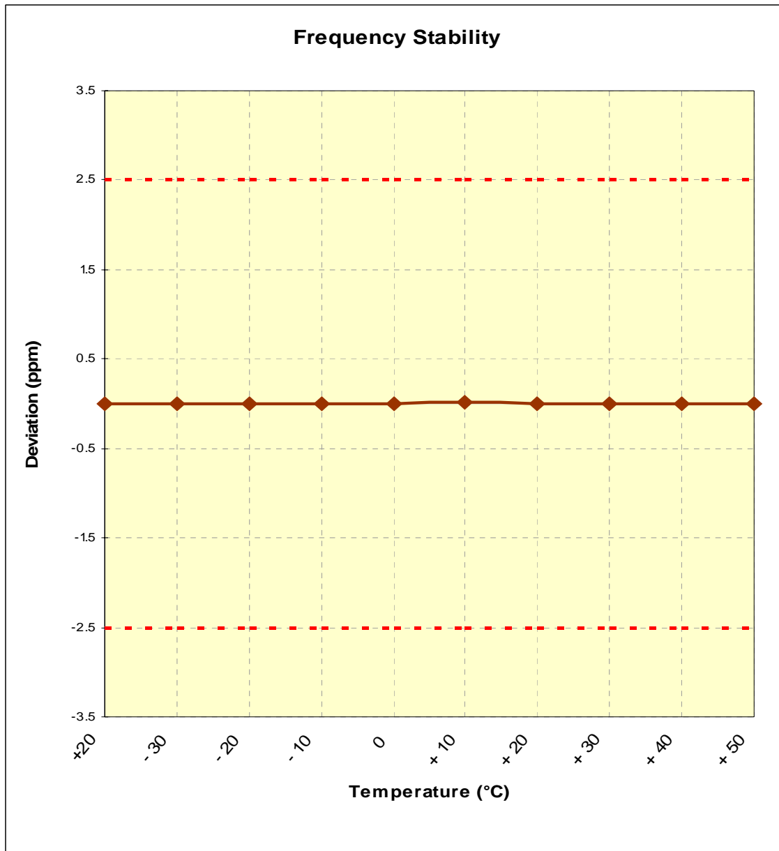
Figure 6-3. Frequency Stability Graph (PCS CDMA Mode – Ch. 600)
