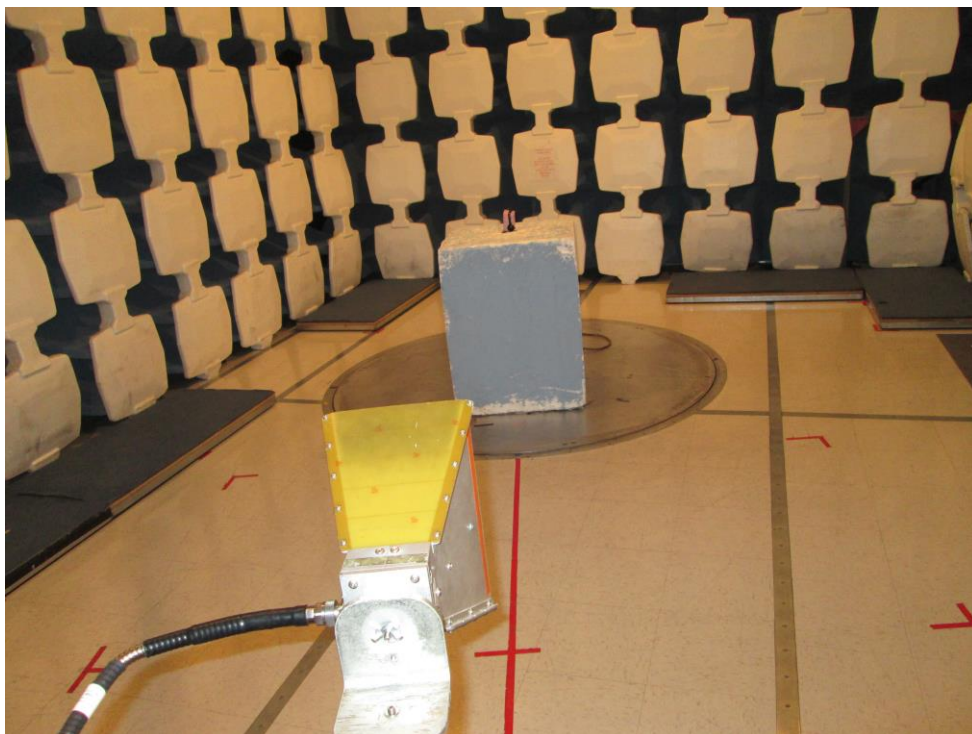
EMI Radiated – 1-6GHz
