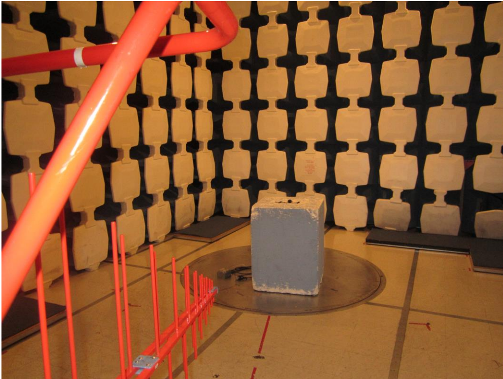
EMI Radiated – 25-1000MHz
