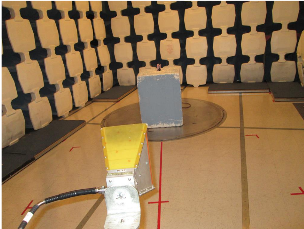
EMI Radiated – Fundamental Frequencies
