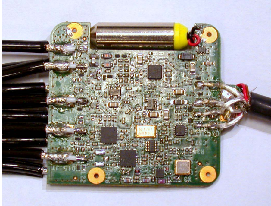
Photograph No. 8 Sensor array PCB second side view
