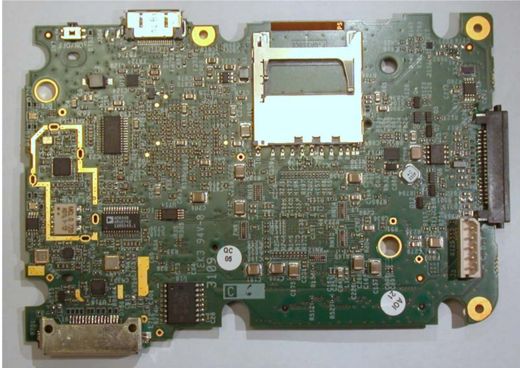
Photograph No. 4 PCB second side view without shielding
