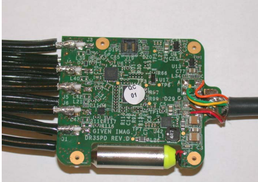
Photograph No. 7 Sensor array PCB front view
