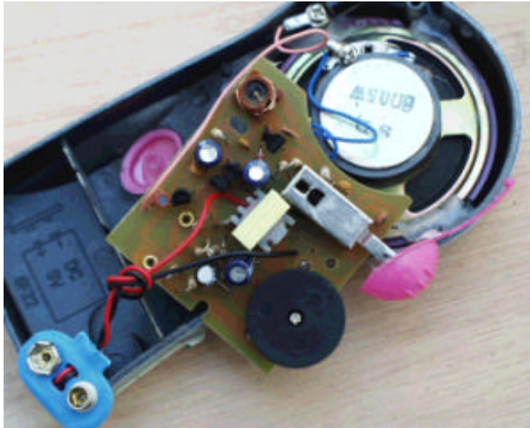
FRONT VIEW OF THE PRINTED WIRING BOARD
