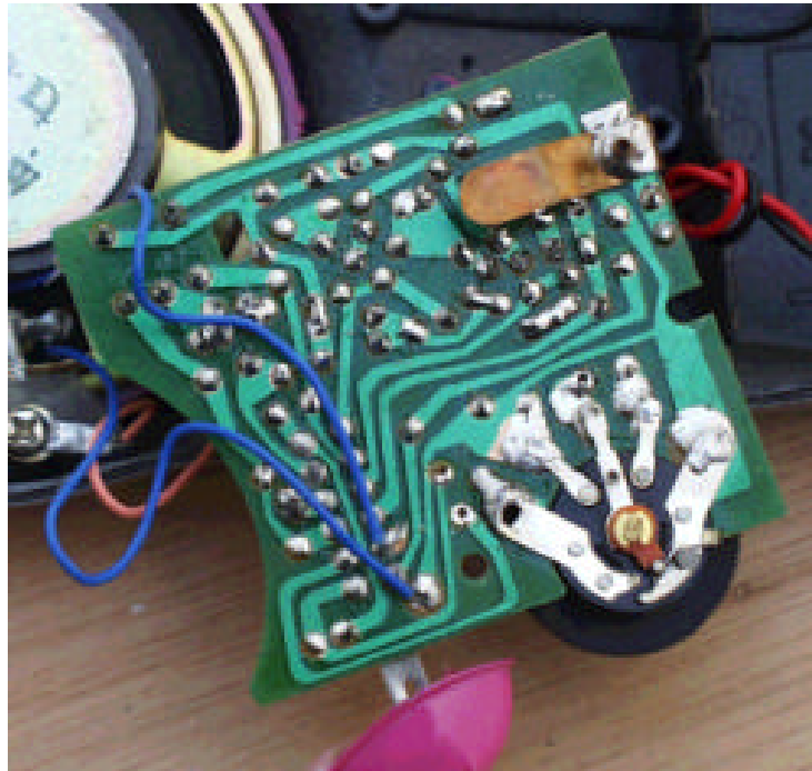
BOTTOM VIEW OF THE PRINTED WIRING BOARD
