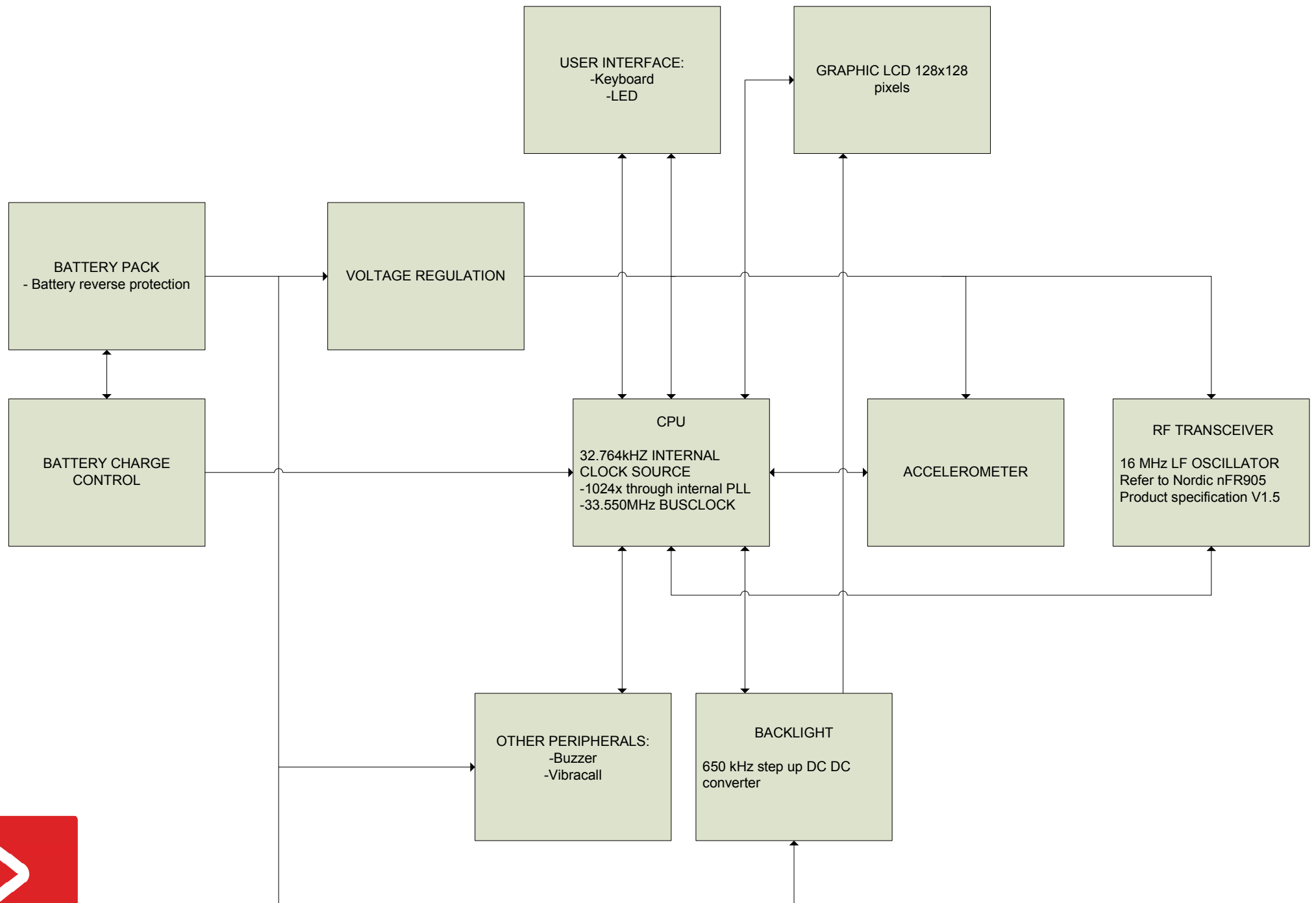
RTX TREND LCD BLOCK DIAGRAM
