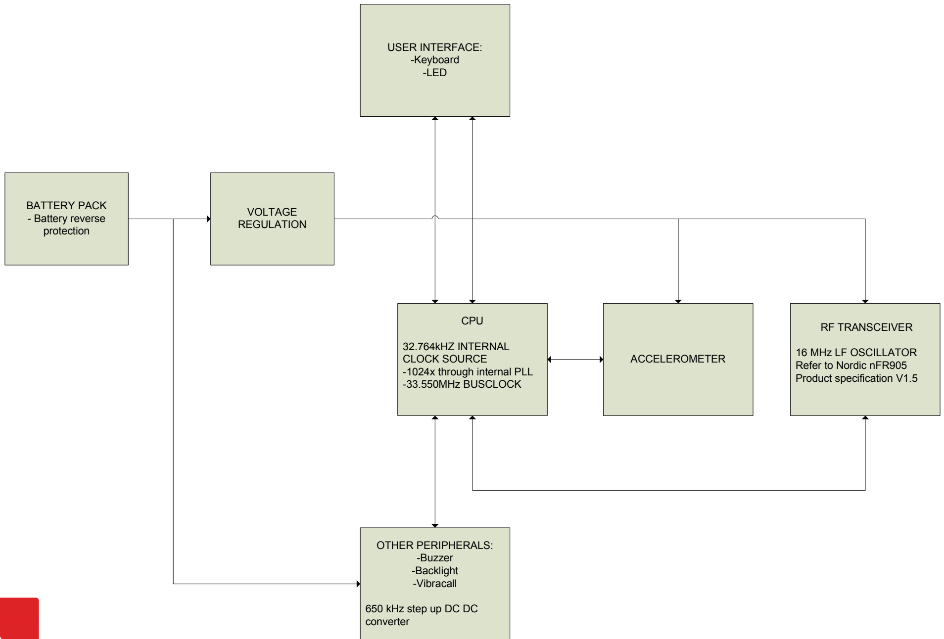
RTX EASY - RTX TREND BLOCK DIAGRAM
