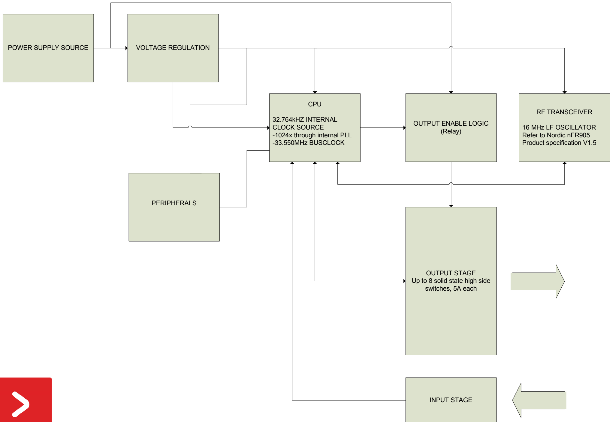
CONTROLLER 8 BLOCK DIAGRAM
