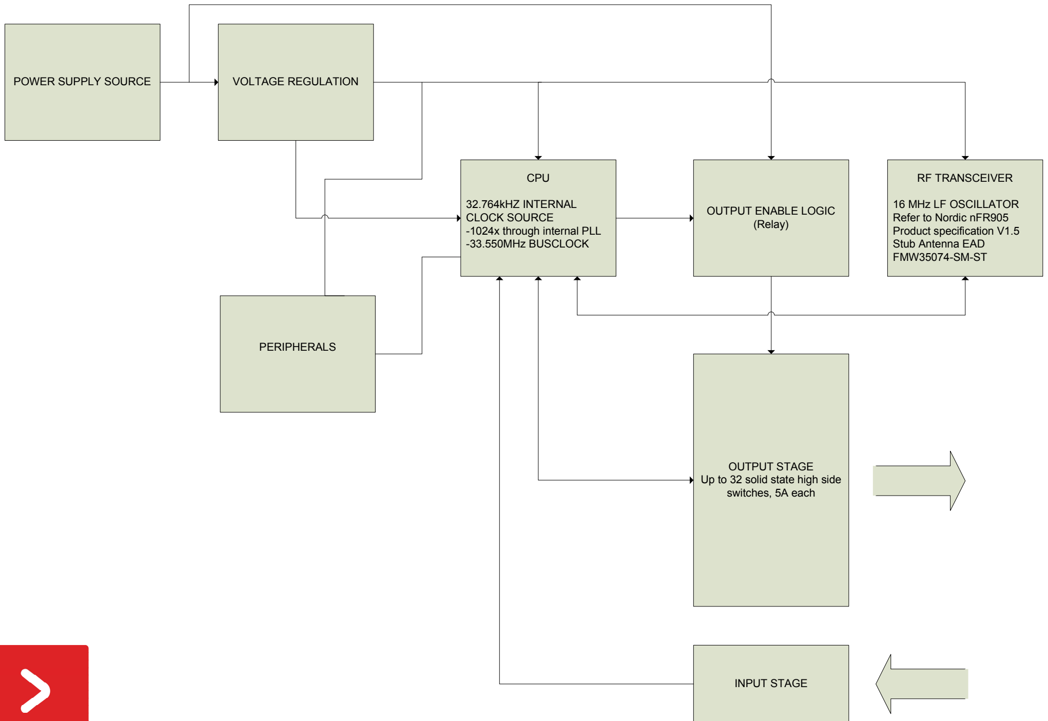
CONTROLLER 32 BLOCK DIAGRAM
