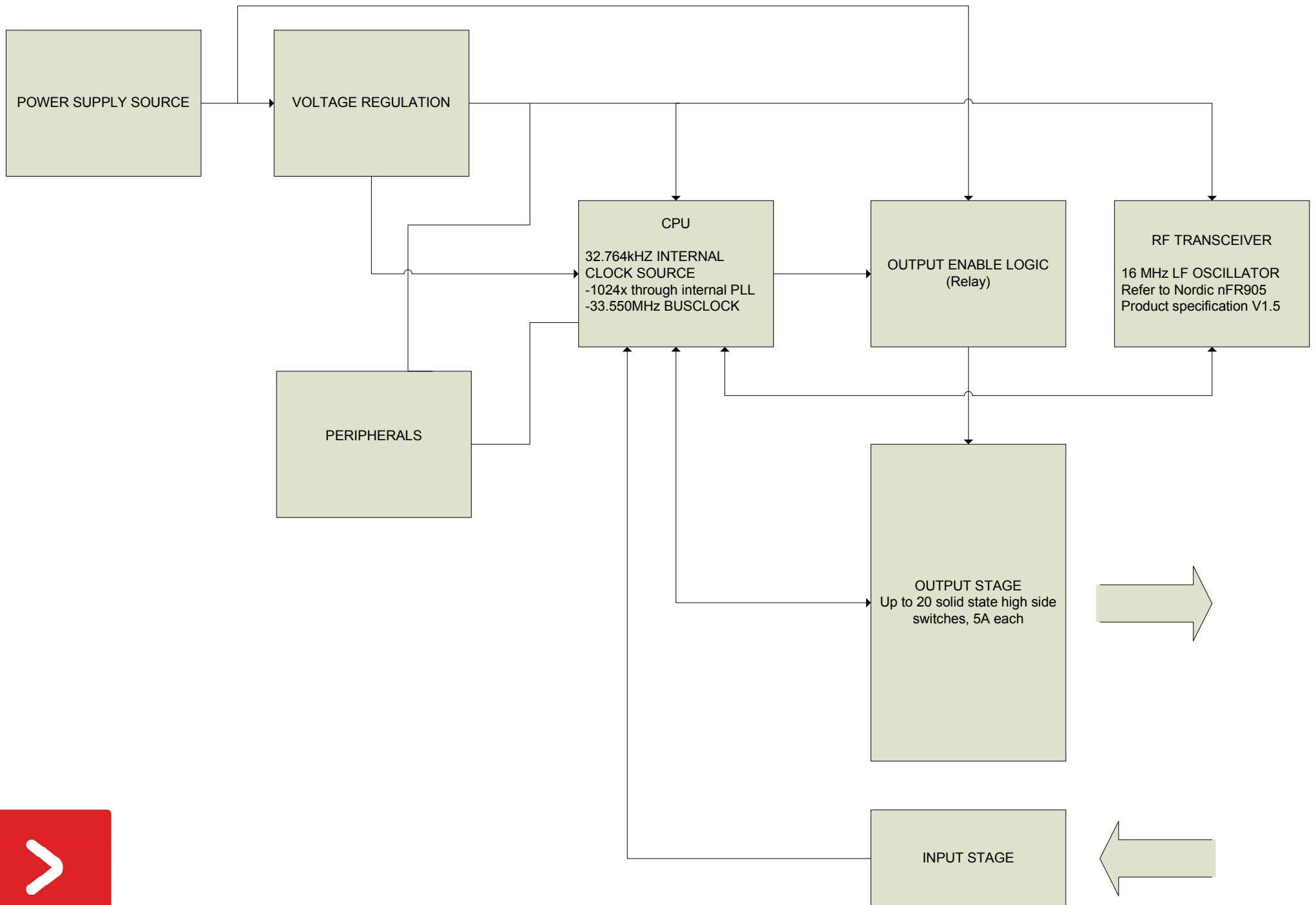
CONTROLLER 20 BLOCK DIAGRAM
