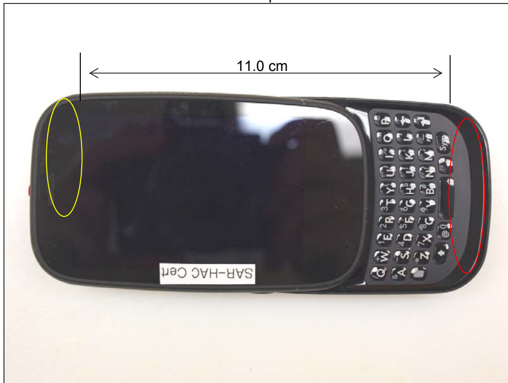
Slide open
