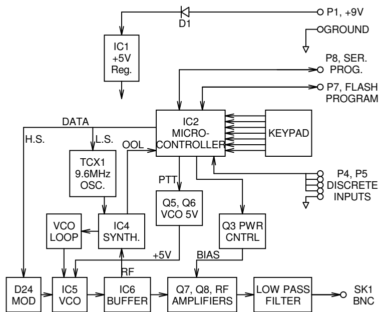
11-85 UHF POCSAG TRANSMITTER
