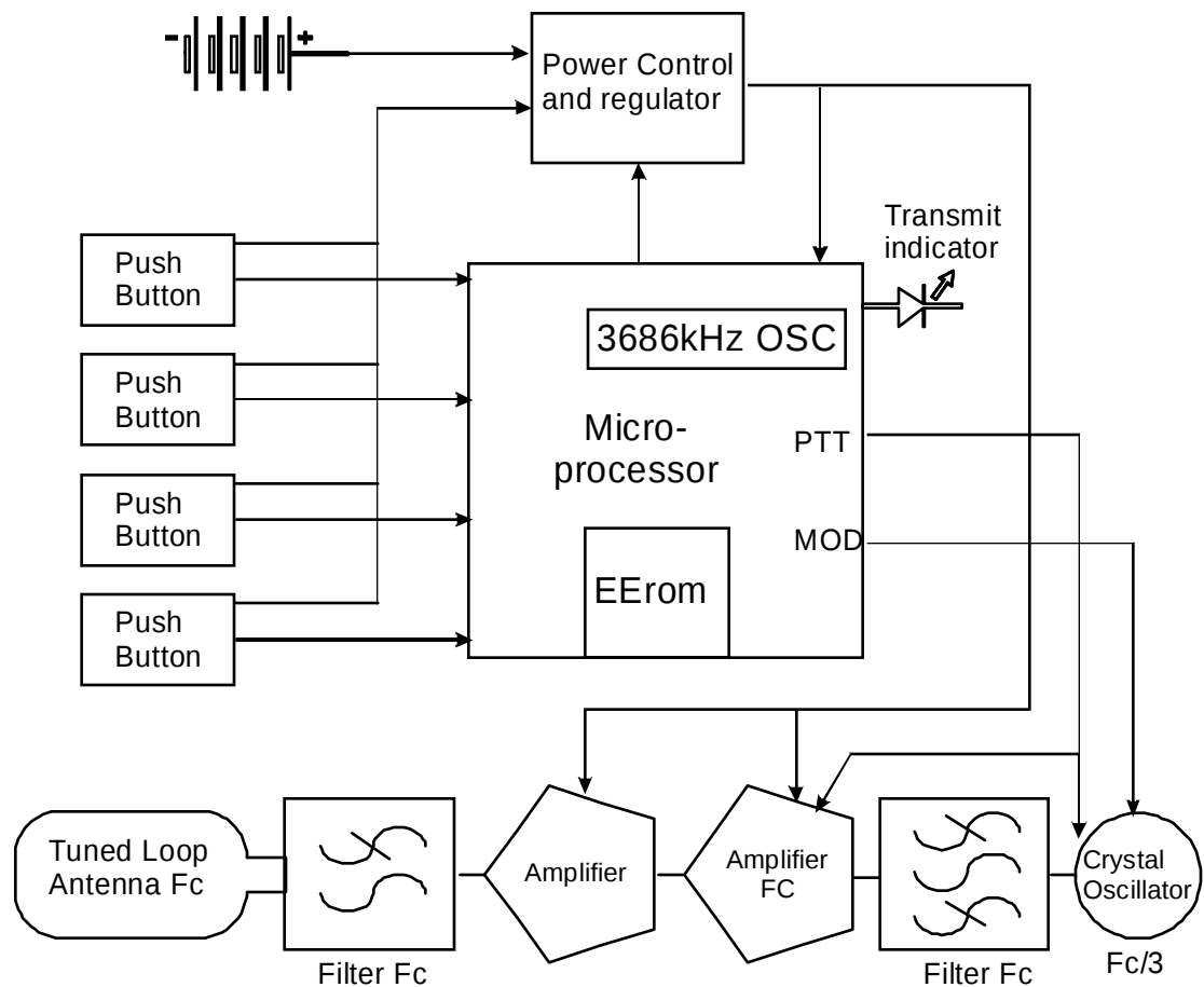
Block Diagram of SALCOM 1167, 1170, 1187, 1143
