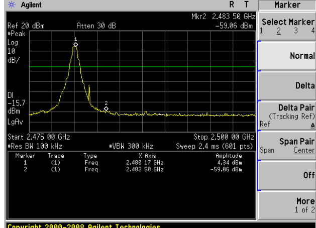
BDR mode (GFSK): Band Edge-High Channel (Hopping Mode)
