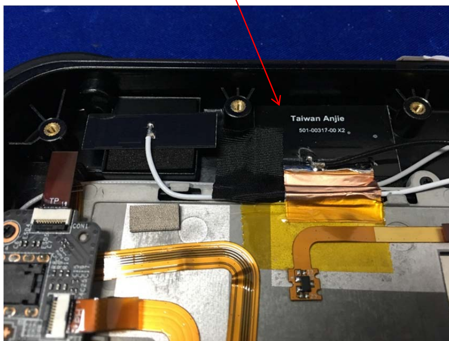
WIFI(Aux Antenna)
