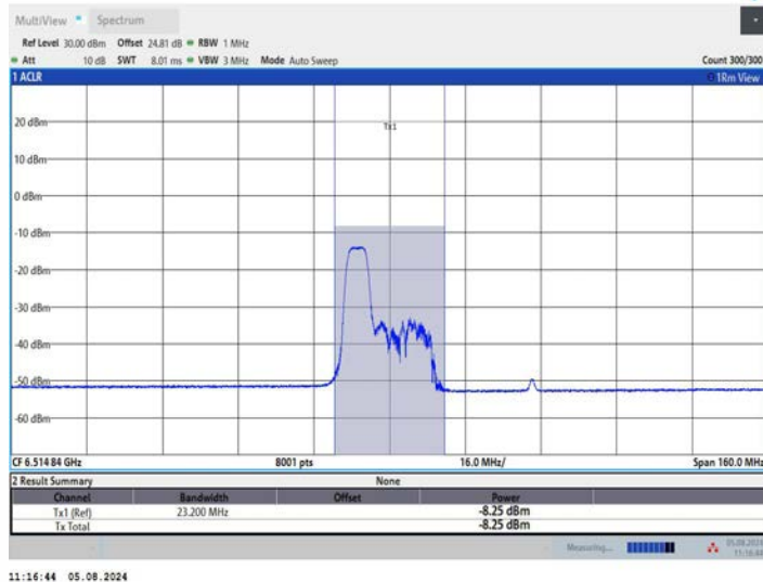
11AX80MIMO_Ant1_6545_106Tone_RU53
