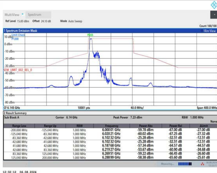
11AX80MIMO_Ant1_6145_106Tone_RU53
