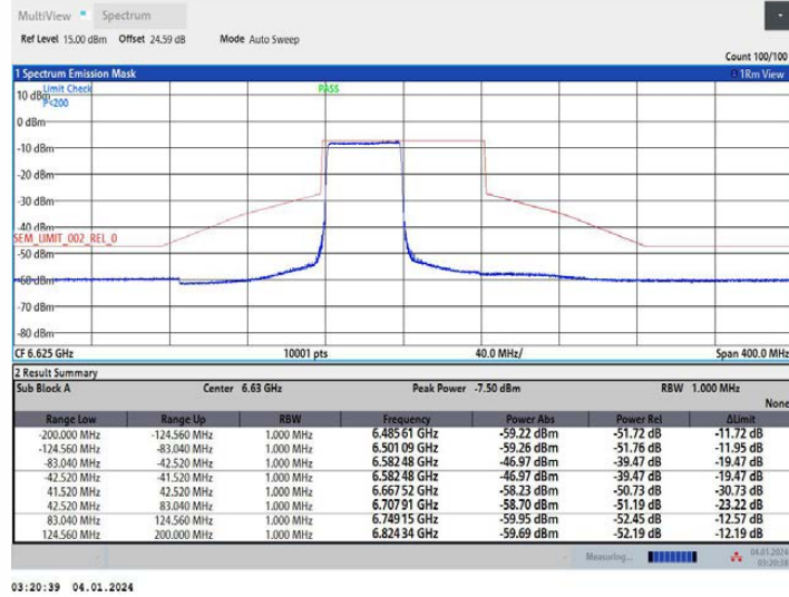
11AX80MIMO Ant1_6625_26Tone_RU0
