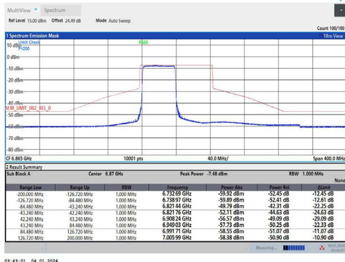
11AX80MIMO Ant1_6865_26Tone_RU0
