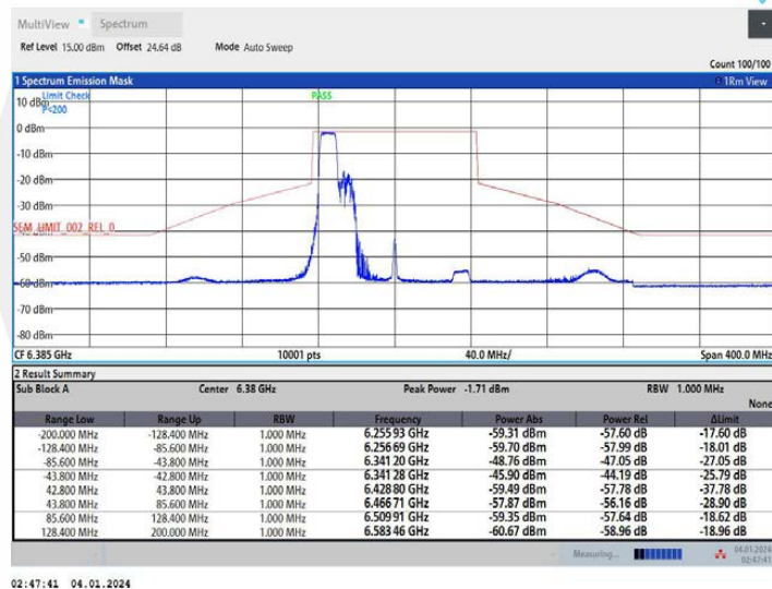
11AX80MIMO Ant1 6385_242Tone RU61
