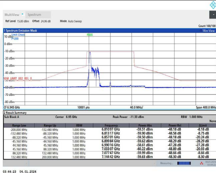
11AX80MIMO Ant1 6945 52Tone RU37
