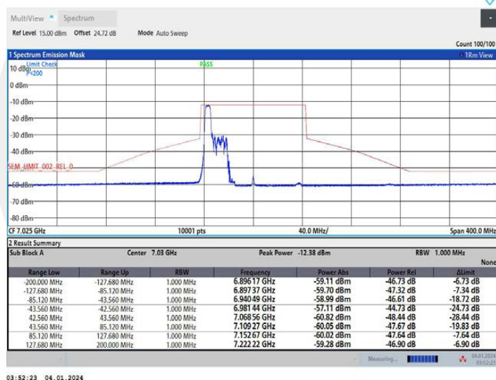
11AX80MIMO Ant2 7025 106Tone RU53
