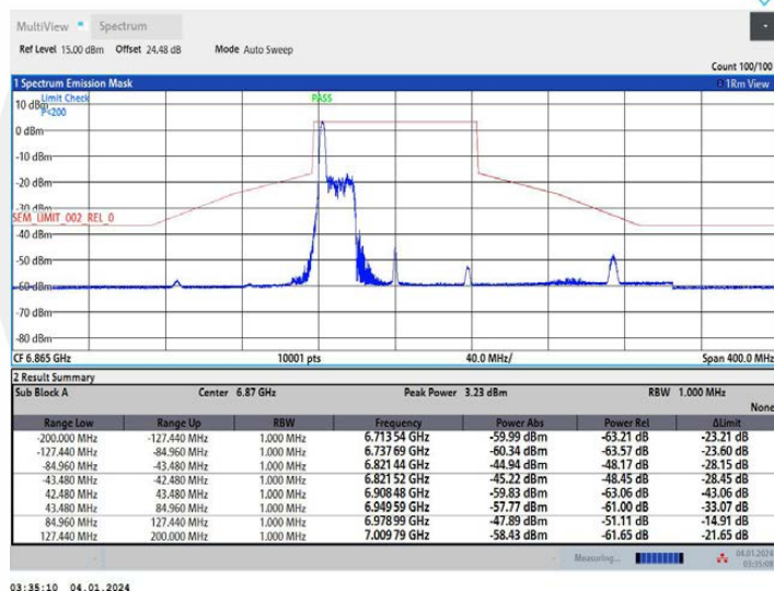
11AX80MIMO Ant1_6865_52Tone_RU37
