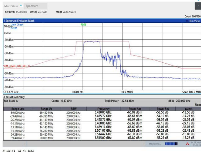
11AX20MIMO Ant1_6475_26Tone_RU0
