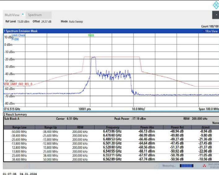
11AX20MIMO Ant1_6515_52Tone_RU37
