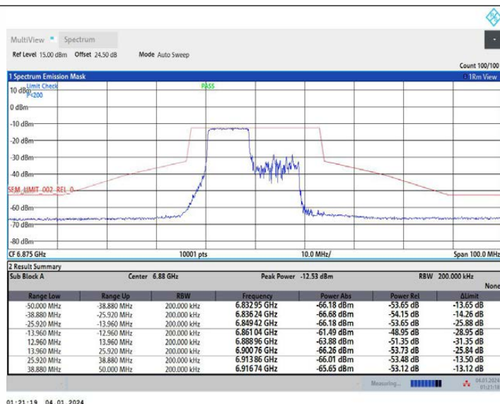
11AX20MIMO Ant1_6875_26Tone_RU0
