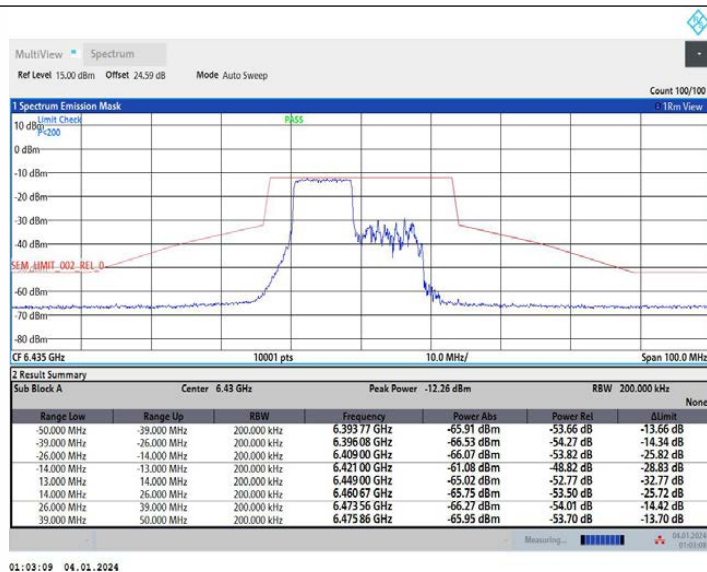
11AX20MIMO Ant1_6435_26Tone_RU0
