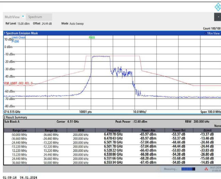
11AX20MIMO Ant1_6515_26Tone_RU0
