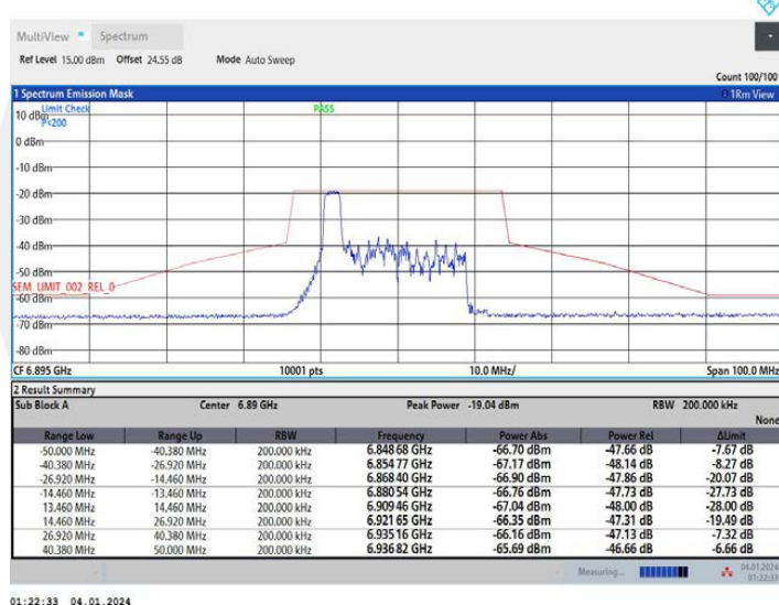
11AX20MIMO Ant1_6895_52Tone_RU37
