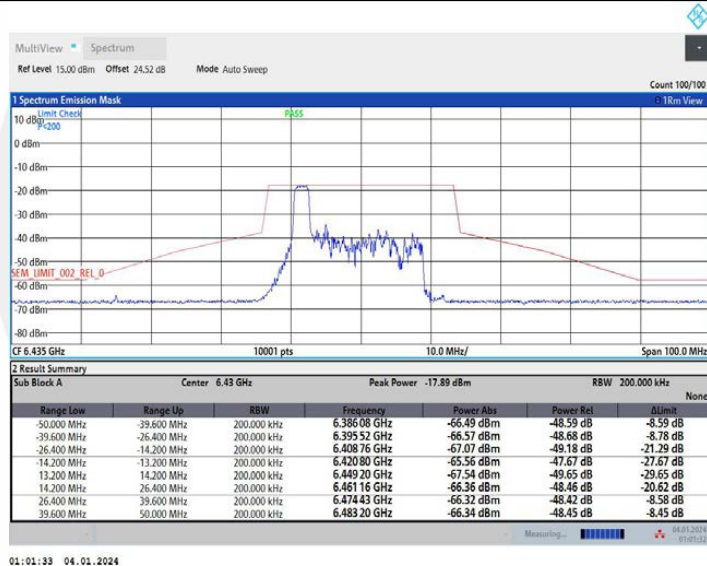
11AX20MIMO Ant1_6435_52Tone_RU37
