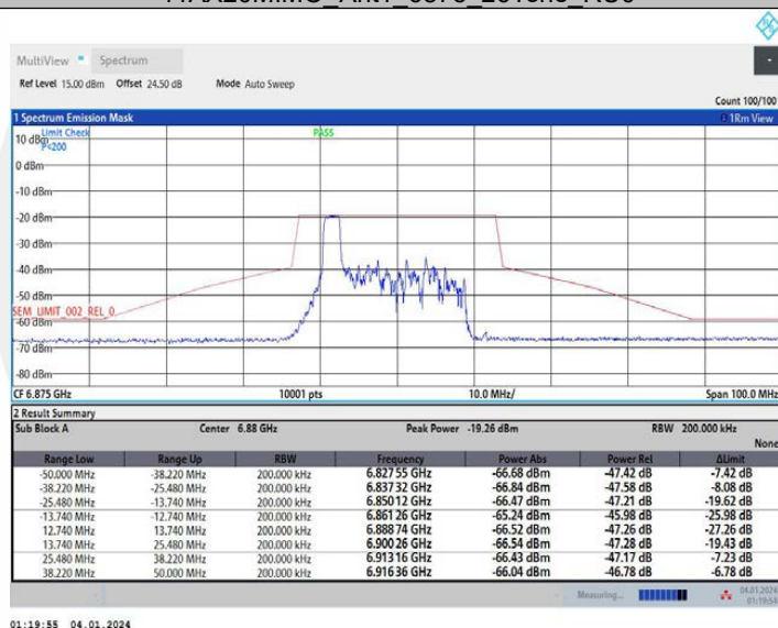
11AX20MIMO Ant1_6875_52Tone_RU37
