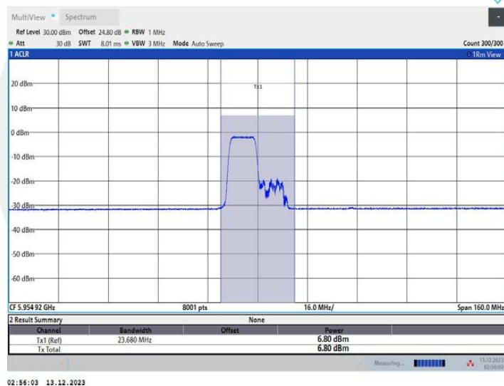
11AX80MIMO Ant1 5985 242Tone RU61
