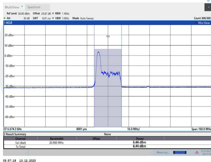
11AX80MIMO Ant1_6705_52Tone_RU37
