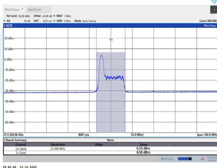
11AX80MIMO Ant1_6625_52Tone_RU37
