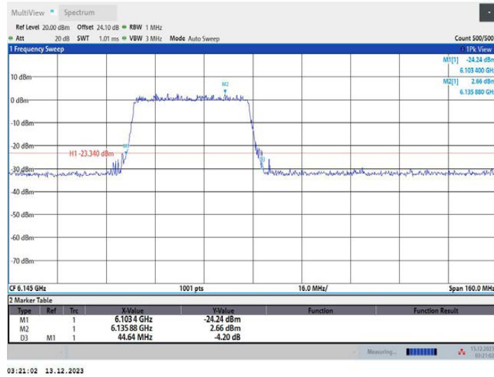
11AX80MIMO_Ant1_6145_26Tone_RU0
