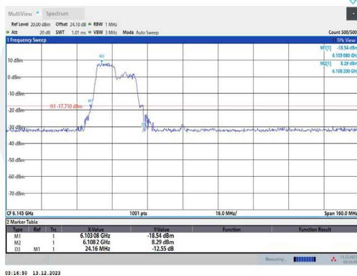
11AX80MIMO_Ant1_6145_242Tone_RU61
