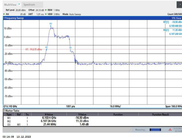
11AX80MIMO_Ant1_6145_106Tone_RU53
