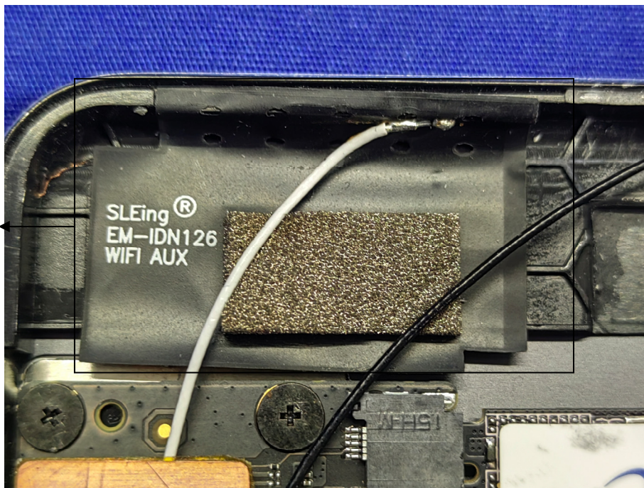
AUX FPC Antenna
