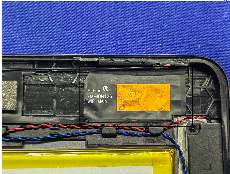
Main FPC Antenna
