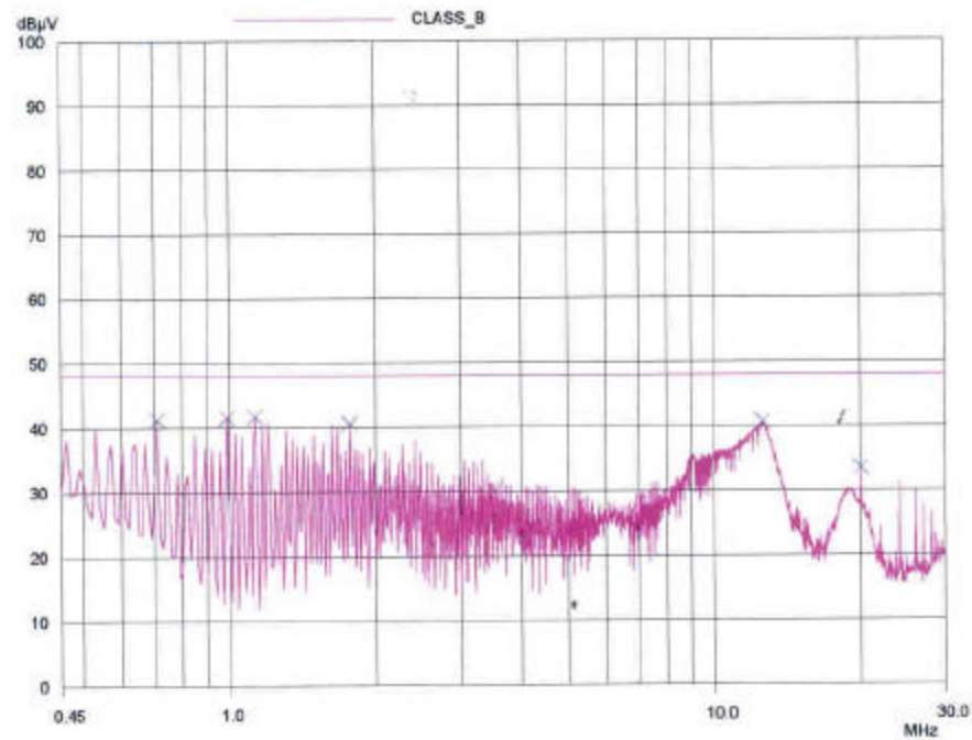
HOT LINE
