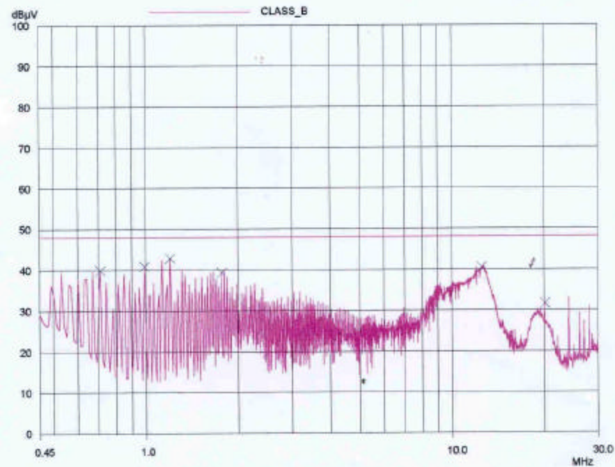
NEUTRAL LINE
