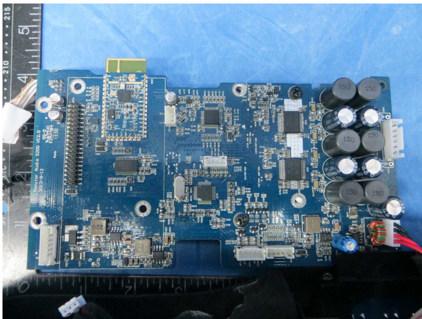
PCB Board
