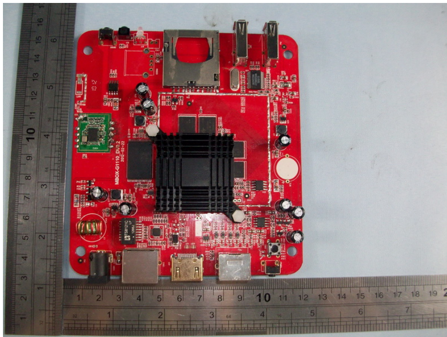
Motherboard top view #1
