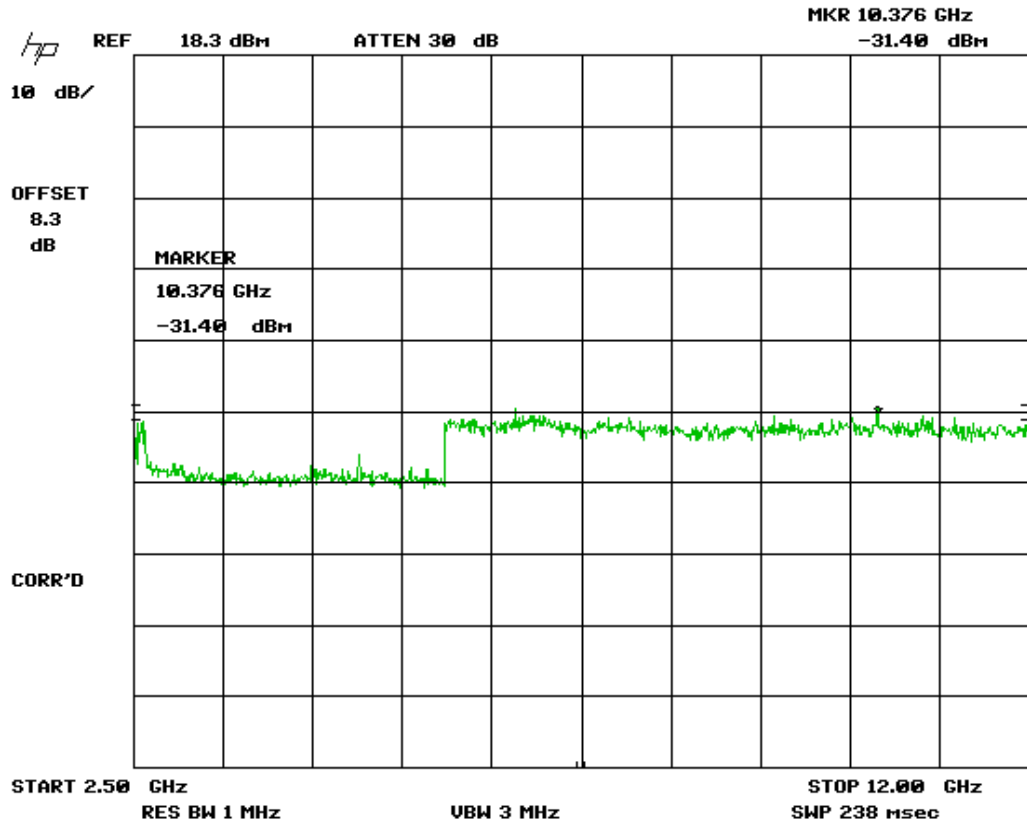
Figure 14. Emissions 802.11b - High Channel, Part 3
